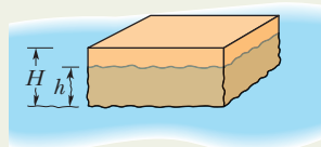
Fig. 14-11 Block of height H floats in a fluid, to a depth of h .
