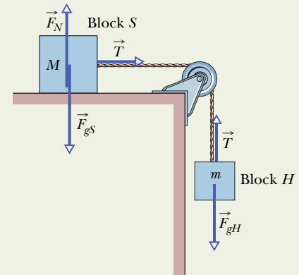
Fig. 5-13 The forces acting on the two blocks of Fig. 5-12.
