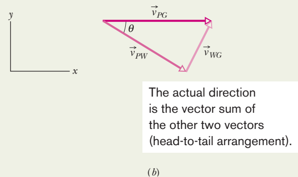
Fig. 4-20 A plane flying in a wind.
