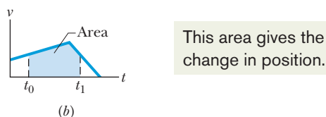
Fig. 2-12 The area between a plotted curve and the horizontal time axis, from time t_0 to time t_1 , is indicated for (a) a graph of acceleration a versus t and (b) a graph of velocity v versus t .
