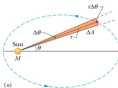
Fig. 13-13 (a) In time \Delta t , the line r connecting the planet to the Sun moves through an angle \Delta\theta , sweeping out an area \Delta A (shaded). (b) The linear momentum \vec{p} of the planet and the components of \vec{p} .
