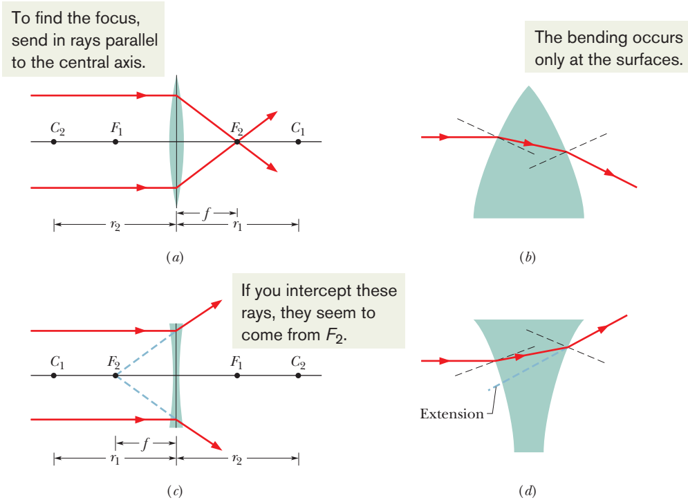
Fig. 34-14 (a) Rays initially parallel to the central axis of a converging lens are made to converge to a real focal point F_2 by the lens. The lens is thinner than drawn, with a width like that of the vertical line through it. We shall consider all the bending of rays as occurring at this central line. (b) An enlargement of the top part of the lens of (a); normals to the surfaces are shown dashed. Note that both refractions bend the ray downward, toward the central axis. (c) The same initially parallel rays are made to diverge by a diverging lens. Extensions of the diverging rays pass through a virtual focal point F_2 . (d) An enlargement of the top part of the lens of (c). Note that both refractions bend the ray upward, away from the central axis.
