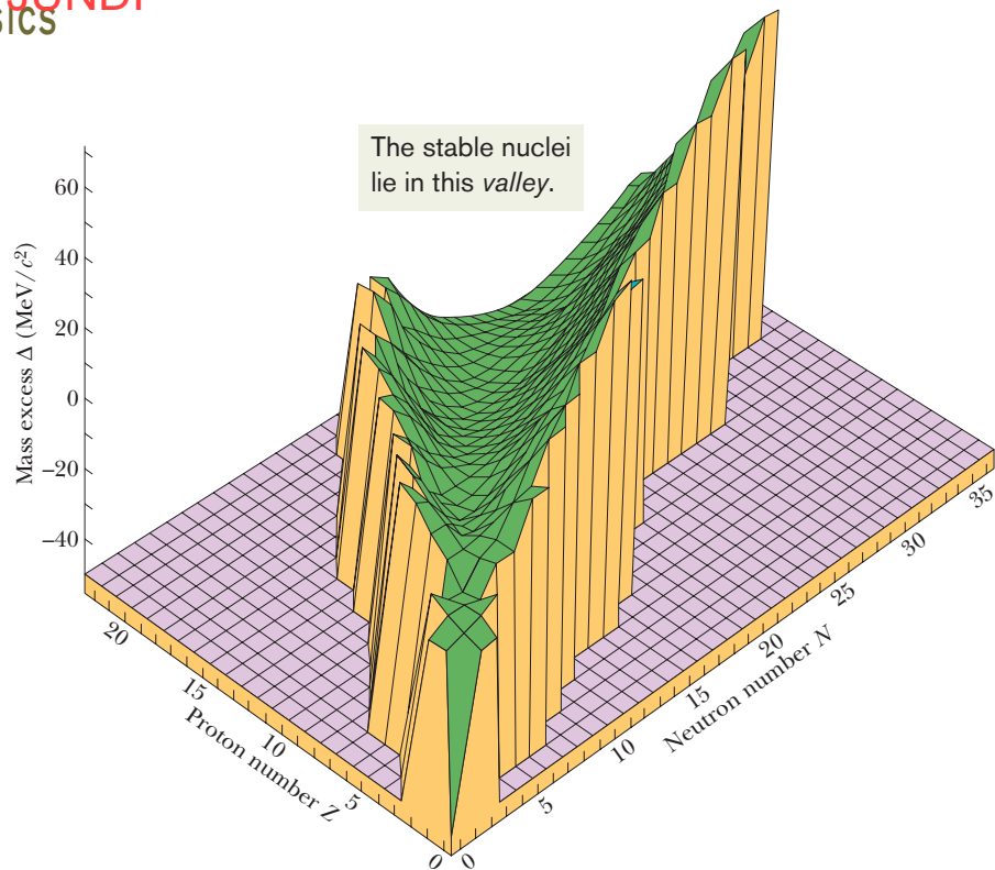
Fig. 42-13 A portion of the valley of the nuclides, showing only the nuclides of low mass. Deuterium, tritium, and helium lie at the near end of the plot, with helium at the high point. The valley stretches away from us, with the plot stopping at about Z = 22 and N = 35 . Nuclides with large values of A , which would be plotted much beyond the valley, can decay into the valley by repeated alpha emissions and by fission (splitting of a nuclide).
