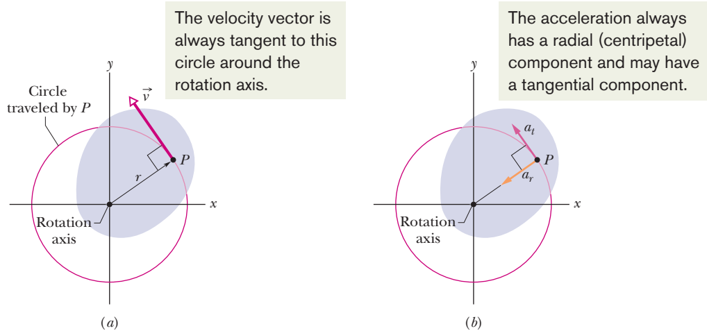
Fig. 10-9 The rotating rigid body of Fig. 10-2, shown in cross section viewed from above. Every point of the body (such as P ) moves in a circle around the rotation axis. (a) The linear velocity \vec{v} of every point is tangent to the circle in which the point moves. (b) The linear acceleration \vec{a} of the point has (in general) two components: tangential a_t and radial a_r .
