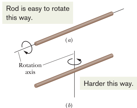
Fig. 10-11 A long rod is much easier to rotate about (a) its central (longitudinal) axis than about (b) an axis through its center and perpendicular to its length. The reason for the difference is that the mass is distributed closer to the rotation axis in (a) than in (b).
