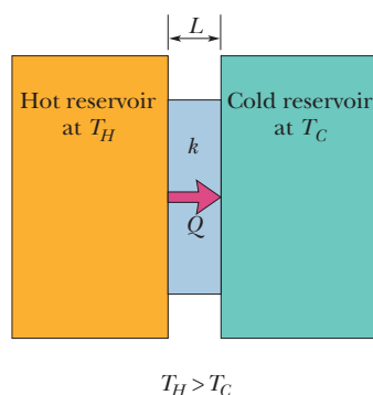
Fig. 18-18 Thermal conduction. Energy is transferred as heat from a reservoir at temperature T_H to a cooler reservoir at temperature T_C through a conducting slab of thickness L and thermal conductivity k .
