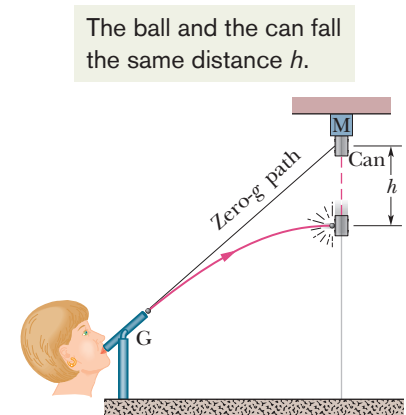
Fig. 4-11 The projectile ball always hits the falling can. Each falls a distance h from where it would be were there no free-fall acceleration.
