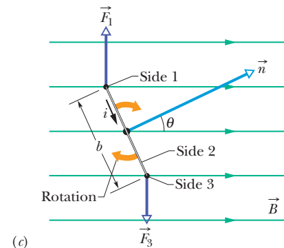
Fig. 28-19 A rectangular loop, of length a and width b and carrying a current i , is located in a uniform magnetic field. A torque \tau acts to align the normal vector \vec{n} with the direction of the field. (a) The loop as seen by looking in the direction of the magnetic field. (b) A perspective of the loop showing how the right-hand rule gives the direction of \vec{n} , which is perpendicular to the plane of the loop. (c) A side view of the loop, from side 2. The loop rotates as indicated.
