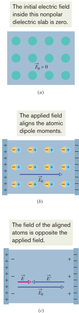
Fig. 25-15 (a) A nonpolar dielectric slab. The circles represent the electrically neutral atoms within the slab. (b) An electric field is applied via charged capacitor plates; the field slightly stretches the atoms, separating the centers of positive and negative charge. (c) The separation produces surface charges on the slab faces. These charges set up a field \vec{E}' , which opposes the applied field \vec{E}_0 . The resultant field \vec{E} inside the dielectric (the vector sum of \vec{E}_0 and \vec{E}' ) has the same direction as \vec{E}_0 but a smaller magnitude.
