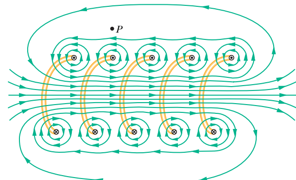
Fig. 29-17 A vertical cross section through the central axis of a “stretched-out” solenoid. The back portions of five turns are shown, as are the magnetic field lines due to a current through the solenoid. Each turn produces circular magnetic field lines near itself. Near the solenoid’s axis, the field lines combine into a net magnetic field that is directed along the axis. The closely spaced field lines there indicate a strong magnetic field. Outside the solenoid the field lines are widely spaced; the field there is very weak.
