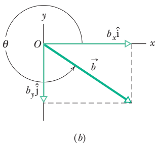
Fig. 3-14 (a) The vector components of vector \vec{a} . (b) The vector components of vector \vec{b} .
