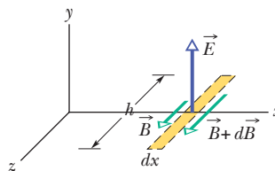
Fig. 33-7 The sinusoidal variation of the electric field through this rectangle, located (but not shown) at point P in Fig. 33-5 b , induces magnetic fields along the rectangle. The instant shown is that of Fig. 33-6: \vec{E} is decreasing in magnitude, and the magnitude of the induced magnetic field is greater on the right side of the rectangle than on the left.
