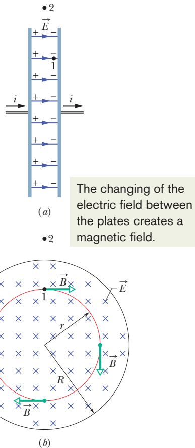
Fig. 32-5 (a) A circular parallel-plate capacitor, shown in side view, is being charged by a constant current i . (b) A view from within the capacitor, looking toward the plate at the right in (a). The electric field \vec{E} is uniform, is directed into the page (toward the plate), and grows in magnitude as the charge on the capacitor increases. The magnetic field \vec{B} induced by this changing electric field is shown at four points on a circle with a radius r less than the plate radius R .
