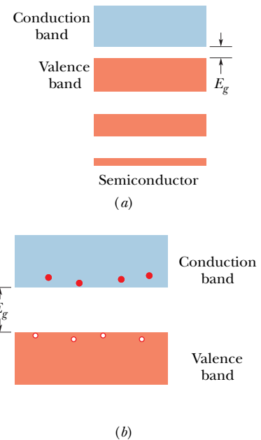
Fig. 41-9 (a) The band-gap pattern for a semiconductor. It resembles that of an insulator (see Fig. 41-4) except that here the energy gap E_g is much smaller; thus electrons, because of their thermal agitation, have some reasonable probability of being able to jump the gap. (b) Thermal agitation has caused a few electrons to jump the gap from the valence band to the conduction band, leaving an equal number of holes in the valence band.
