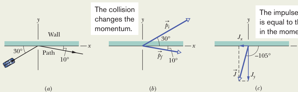
Fig. 9-11 (a) Overhead view of the path taken by a race car and its driver as the car slams into the racetrack wall. (b) The initial momentum \vec{p}_i and final momentum \vec{p}_f of the driver. (c) The impulse \vec{J} on the driver during the collision.
