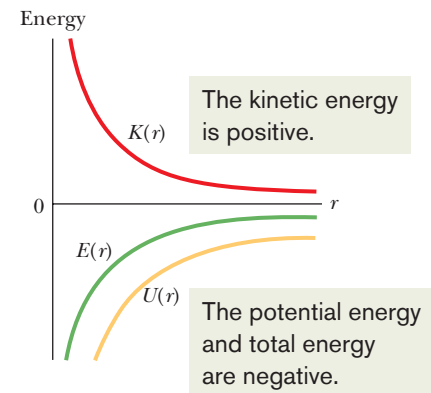
Fig. 13-16 The variation of kinetic energy K , potential energy U , and total energy E with radius r for a satellite in a circular orbit. For any value of r , the values of U and E are negative, the value of K is positive, and E = -K . As r \rightarrow \infty , all three energy curves approach a value of zero.
