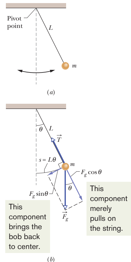
Fig. 15-9 (a) A simple pendulum. (b) The forces acting on the bob are the gravitational force \vec{F}_g and the force \vec{T} from the string. The tangential component F_g \sin \theta of the gravitational force is a restoring force that tends to bring the pendulum back to its central position.
