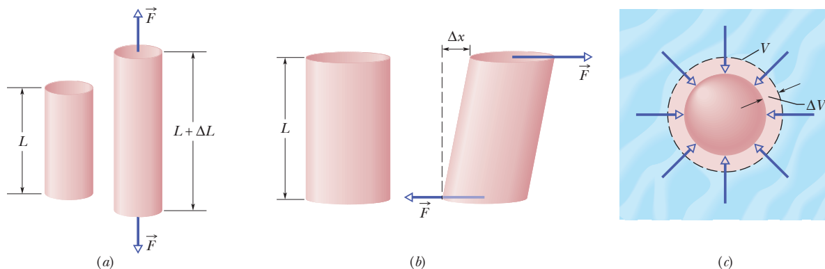
Fig. 12-10 ( a ) A cylinder subject to tensile stress stretches by an amount \Delta L . ( b ) A cylinder subject to shearing stress deforms by an amount \Delta x , somewhat like a pack of playing cards would. ( c ) A solid sphere subject to uniform hydraulic stress from a fluid shrinks in volume by an amount \Delta V . All the deformations shown are greatly exaggerated.
