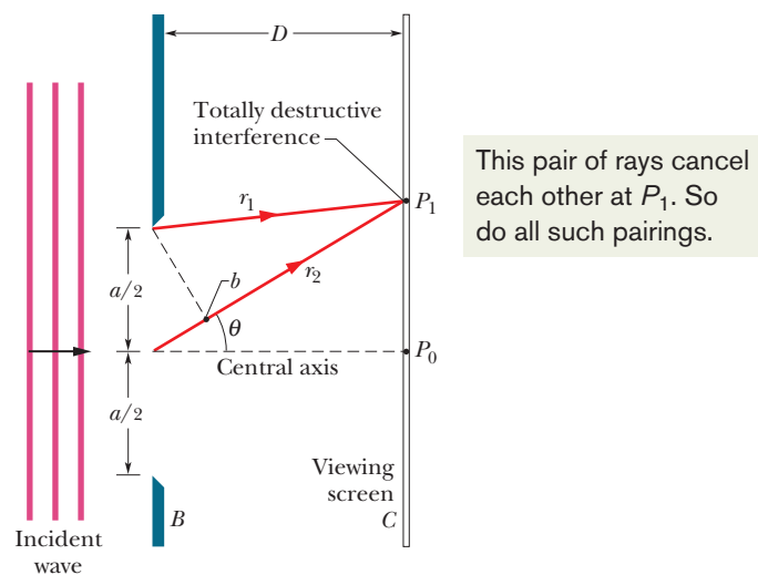
Fig. 36-4 Waves from the top points of two zones of width a/2 undergo fully destructive interference at point P_1 on viewing screen C .
