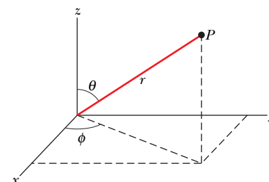
Fig. 39-22 The relationship between the coordinates x, y, and z of the rectangular coordinate system and the coordinates r, \theta, and \phi of the spherical coordinate system. The latter are more appropriate for analyzing situations involving spherical symmetry, such as the hydrogen atom.
