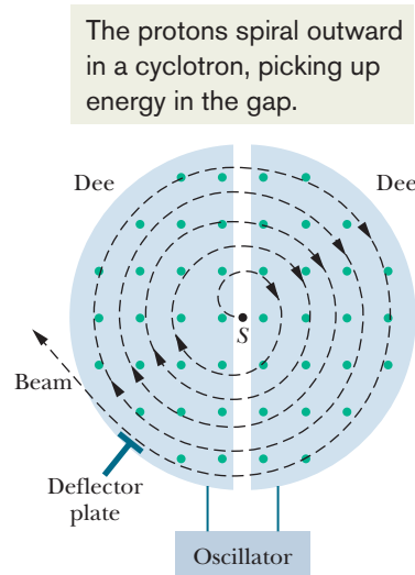
Fig. 28-13 The elements of a cyclotron, showing the particle source S and the dees. A uniform magnetic field is directed up from the plane of the page. Circulating protons spiral outward within the hollow dees, gaining energy every time they cross the gap between the dees.
