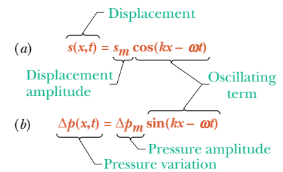
Fig. 17-5 (a) The displacement function and (b) the pressure-variation function of a traveling sound wave consist of an amplitude and an oscillating term.
