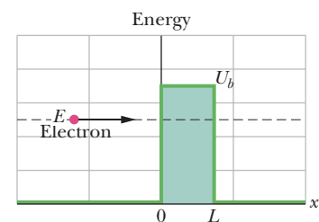
Fig. 38-15 An energy diagram containing two plots for the situation of Fig. 38-13: (1) The electron's mechanical energy E is plotted when the electron is at any coordinate x < 0 . (2) The electron's electric potential energy U is plotted as a function of the electron's position x , assuming that the electron can reach any value of x . The nonzero part of the plot (the potential barrier) has height U_b and thickness L .
