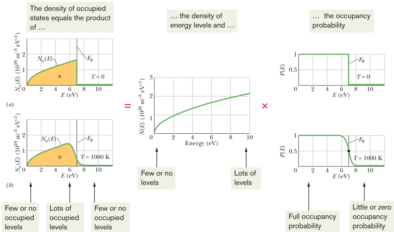
Fig. 41-8 (a) The density of occupied states N_o(E) for copper at absolute zero. The area under the curve is the number density of electrons n . Note that all states with energies up to the Fermi energy E_F = 7 eV are occupied, and all those with energies above the Fermi energy are vacant. (b) The same for copper at T = 1000 K. Note that only electrons with energies near the Fermi energy have been affected and redistributed.
