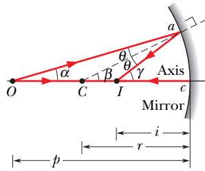
Fig. 34-22 A concave spherical mirror forms a real point image I by reflecting light rays from a point object O .
