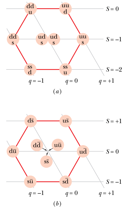
Fig. 44-4 (a) The quark compositions of the eight spin- \frac{1}{2} baryons plotted in Fig. 44-3a. (Although the two central baryons share the same quark structure, they are different particles. The sigma is an excited state of the lambda, decaying into the lambda by emission of a gamma-ray photon.) (b) The quark compositions of the nine spin-zero mesons plotted in Fig. 44-3b.
