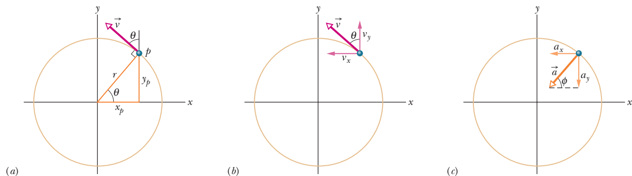
Fig. 4-17 Particle p moves in counterclockwise uniform circular motion. (a) Its position and velocity \vec{v} . (b) Velocity \vec{v} . (c) Acceleration \vec{a} .
