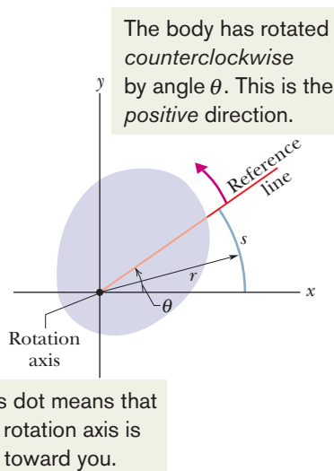
Fig. 10-3 The rotating rigid body of Fig. 10-2 in cross section, viewed from above. The plane of the cross section is perpendicular to the rotation axis, which now extends out of the page, toward you. In this position of the body, the reference line makes an angle \theta with the x axis.
