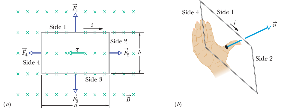
Fig. 28-19 A rectangular loop, of length a and width b and carrying a current i , is located in a uniform magnetic field. A torque \tau acts to align the normal vector \vec{n} with the direction of the field. (a) The loop as seen by looking in the direction of the magnetic field. (b) A perspective of the loop showing how the right-hand rule gives the direction of \vec{n} , which is perpendicular to the plane of the loop. (c) A side view of the loop, from side 2. The loop rotates as indicated.
