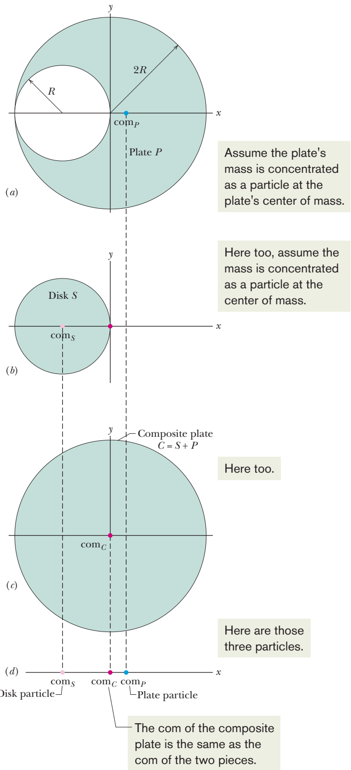
Fig. 9-3 (a) Plate P is a metal plate of radius 2R , with a circular hole of radius R . The center of mass of P is at point com_P . (b) Disk S . (c) Disk S has been put back into place to form a composite plate C . The center of mass com_S of disk S and the center of mass com_C of plate C are shown. (d) The center of mass com_{S+P} of the combination of S and P coincides with com_C , which is at x = 0 .
