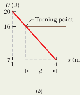
Fig. 8-10 (a) A plot of potential energy U versus position x . (b) A section of the plot used to find where the particle turns around.
