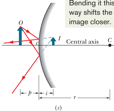
Fig. 34-8 (a) An object O forms a virtual image I in a plane mirror. (b) If the mirror is bent so that it becomes concave , the image moves farther away and becomes larger. (c) If the plane mirror is bent so that it becomes convex , the image moves closer and becomes smaller.
