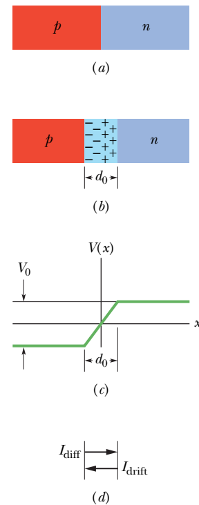
Fig. 41-12 (a) A p-n junction. (b) Motions of the majority charge carriers across the junction plane uncover a space charge associated with uncompensated donor ions (to the right of the plane) and acceptor ions (to the left). (c) Associated with the space charge is a contact potential difference V_0 across d_0 . (d) The diffusion of majority carriers (both electrons and holes) across the junction plane produces a diffusion current I_{\text{diff}} . (In a real p-n junction, the boundaries of the depletion zone would not be sharp, as shown here, and the contact potential curve (c) would be smooth, with no sharp corners.)
