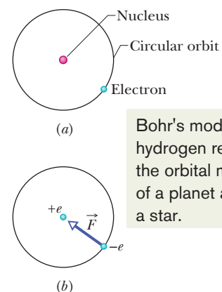
Fig. 39-16 (a) Circular orbit of an electron in the Bohr model of the hydrogen atom. (b) The Coulomb force \vec{F} on the electron is directed radially inward toward the nucleus.
