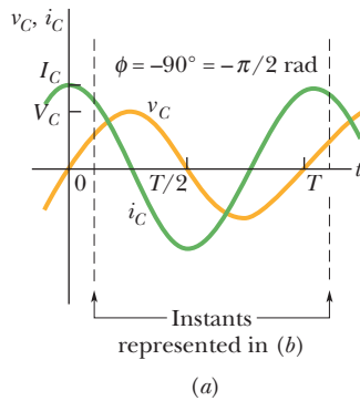
Fig. 31-11 (a) The current in the capacitor leads the voltage by 90^\circ (= \pi/2 \text{ rad}) . (b) A phasor diagram shows the same thing.
