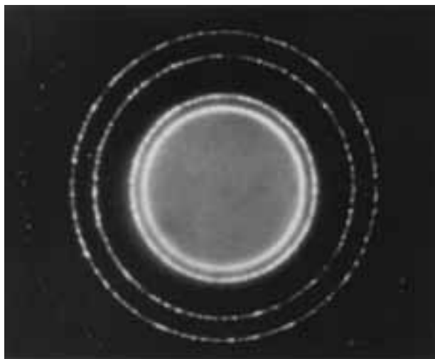
Fig. 38-9 (a) An experimental arrangement used to demonstrate, by diffraction techniques, the wave-like character of the incident beam. Photographs of the diffraction patterns when the incident beam is (b) an x-ray beam (light wave) and (c) an electron beam (matter wave). Note that the two patterns are geometrically identical to each other. (Photo (b) Cameca, Inc. Photo (c) from PSSC film "Matter Waves," courtesy Education Development Center, Newton, Massachusetts)
