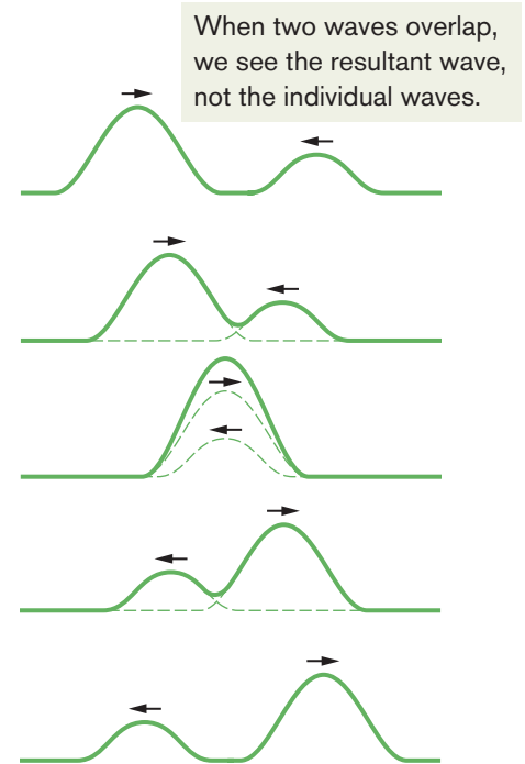
Fig. 16-11 A series of snapshots that show two pulses traveling in opposite directions along a stretched string. The superposition principle applies as the pulses move through each other.
