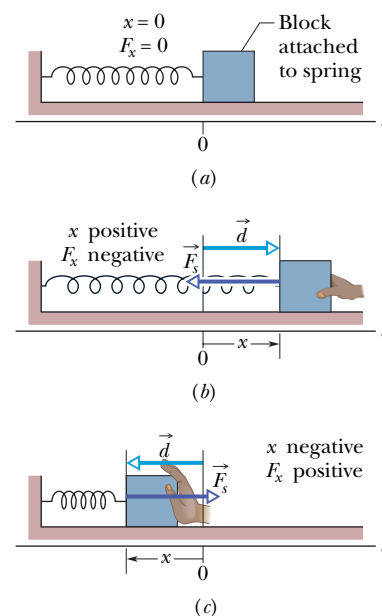
Fig. 7-9 (a) A spring in its relaxed state. The origin of an x axis has been placed at the end of the spring that is attached to a block. (b) The block is displaced by \vec{d} , and the spring is stretched by a positive amount x . Note the restoring force \vec{F}_s exerted by the spring. (c) The spring is compressed by a negative amount x . Again, note the restoring force.
