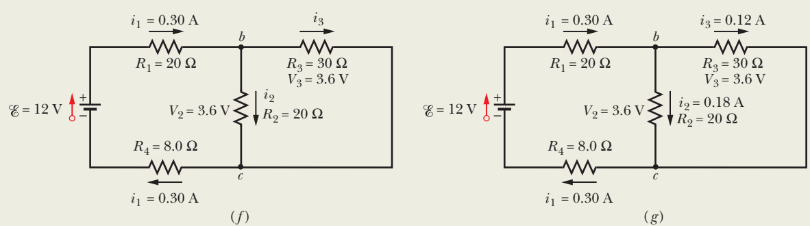
Figure 27-11 (a) A circuit with an ideal battery. (b) Label the currents. (c) Replacing the parallel resistors with their equivalent. (d)–(g) Working backward to find the currents through the parallel resistors.
