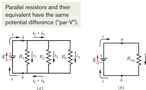
Figure 27-10 (a) Three resistors connected in parallel across points a and b . (b) An equivalent circuit, with the three resistors replaced with their equivalent resistance R_{eq} .
