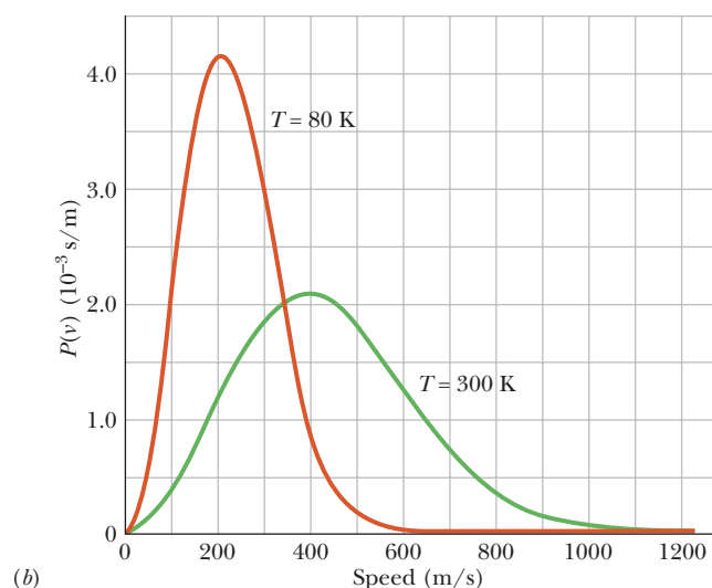
Figure 19-8 (a) The Maxwell speed distribution for oxygen molecules at T = 300 \text{ K} . The three characteristic speeds are marked. (b) The curves for 300 \text{ K} and 80 \text{ K} . Note that the molecules move more slowly at the lower temperature. Because these are probability distributions, the area under each curve has a numerical value of unity.
