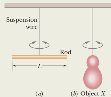
Figure 15-10 Two torsion pendulums, consisting of (a) a wire and a rod and (b) the same wire and an irregularly shaped object.
