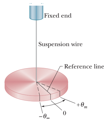
Figure 15-9 A torsion pendulum is an angular version of a linear simple harmonic oscillator. The disk oscillates in a horizontal plane; the reference line oscillates with angular amplitude \theta_m . The twist in the suspension wire stores potential energy as a spring does and provides the restoring torque.
