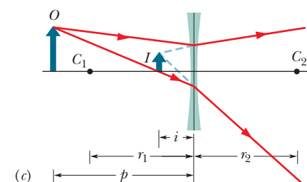
Figure 34-15 (a) A real, inverted image I is formed by a converging lens when the object O is outside the focal point F_1 . (b) The image I is virtual and has the same orientation as O when O is inside the focal point. (c) A diverging lens forms a virtual image I , with the same orientation as the object O , whether O is inside or outside the focal point of the lens.
