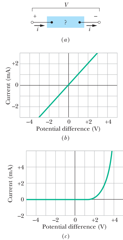
Figure 26-11 (a) A potential difference V is applied to the terminals of a device, establishing a current i . (b) A plot of current i versus applied potential difference V when the device is a 1000 \Omega resistor. (c) A plot when the device is a semiconducting pn junction diode.
