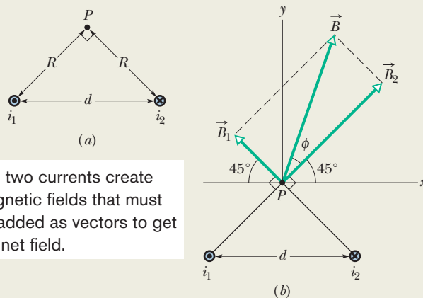
Figure 29-9 (a) Two wires carry currents i_1 and i_2 in opposite directions (out of and into the page). Note the right angle at P. (b) The separate fields \vec{B}_1 and \vec{B}_2 are combined vectorially to yield the net field \vec{B} .
