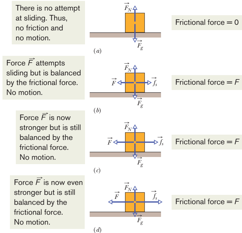
Figure 6-1 (a) The forces on a stationary block. (b–d) An external force \vec{F} , applied to the block, is balanced by a static frictional force \vec{f}_s . As F is increased, f_s also increases, until f_s reaches a certain maximum value. (Figure continues)
