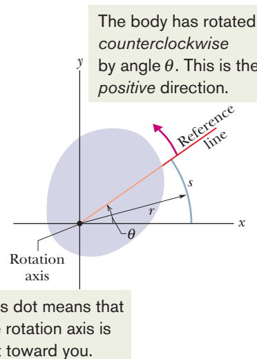
Figure 10-3 The rotating rigid body of Fig. 10-2 in cross section, viewed from above. The plane of the cross section is perpendicular to the rotation axis, which now extends out of the page, toward you. In this position of the body, the reference line makes an angle \theta with the x axis.
