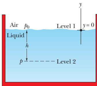
Figure 14-3 The pressure p increases with depth h below the liquid surface according to Eq. 14-8.
