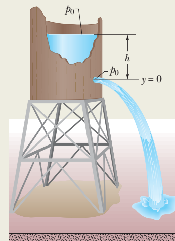
Figure 14-20 Water pours through a hole in a water tank, at a distance h below the water surface. The pressure at the water surface and at the hole is atmospheric pressure p_0 .
