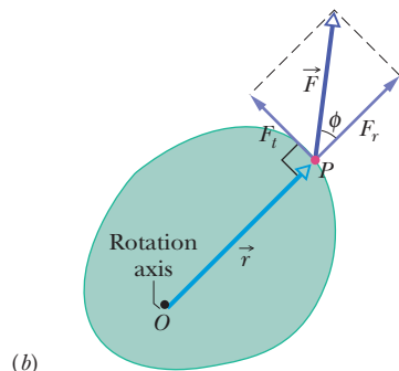
(b) But actually only the tangential component of the force causes the rotation.
