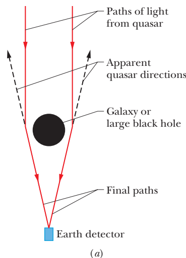
Figure 13-20 (a) Light from a distant quasar follows curved paths around a galaxy or a large black hole because the mass of the galaxy or black hole has curved the adjacent space. If the light is detected, it appears to have originated along the backward extensions of the final paths (dashed lines). (b) The Einstein ring known as MG1131+0456 on the computer screen of a telescope. The source of the light (actually, radio waves, which are a form of invisible light) is far behind the large, unseen galaxy that produces the ring; a portion of the source appears as the two bright spots seen along the ring.
