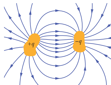
Figure 25-2 Two conductors, isolated electrically from each other and from their surroundings, form a capacitor . When the capacitor is charged, the charges on the conductors, or plates as they are called, have the same magnitude q but opposite signs.
