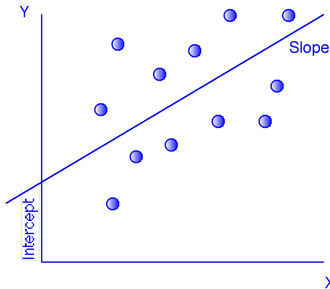
Figure A1.3: Scatter Plot of Y versus X
