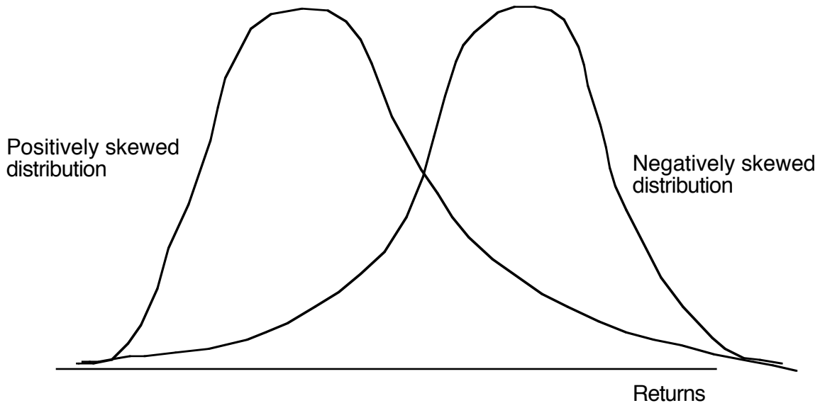
Figure A1.2: Skewed Distributions
