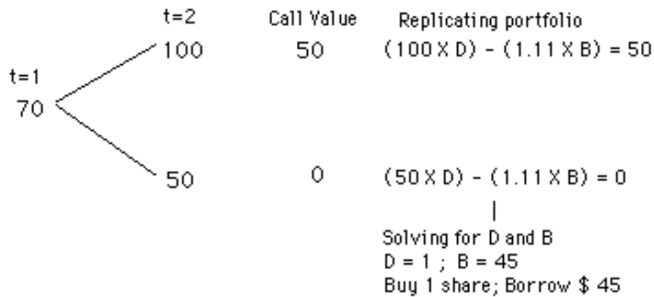
Figure A4.5 Replicating Portfolios When Price Is $ 70
