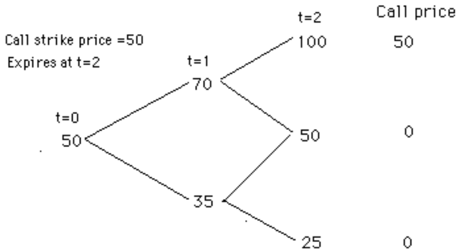
Figure A4.4 Binomial Price Path
