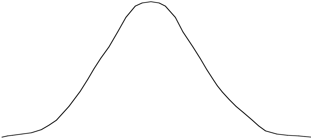
Figure A1.1: Normal Distribution
