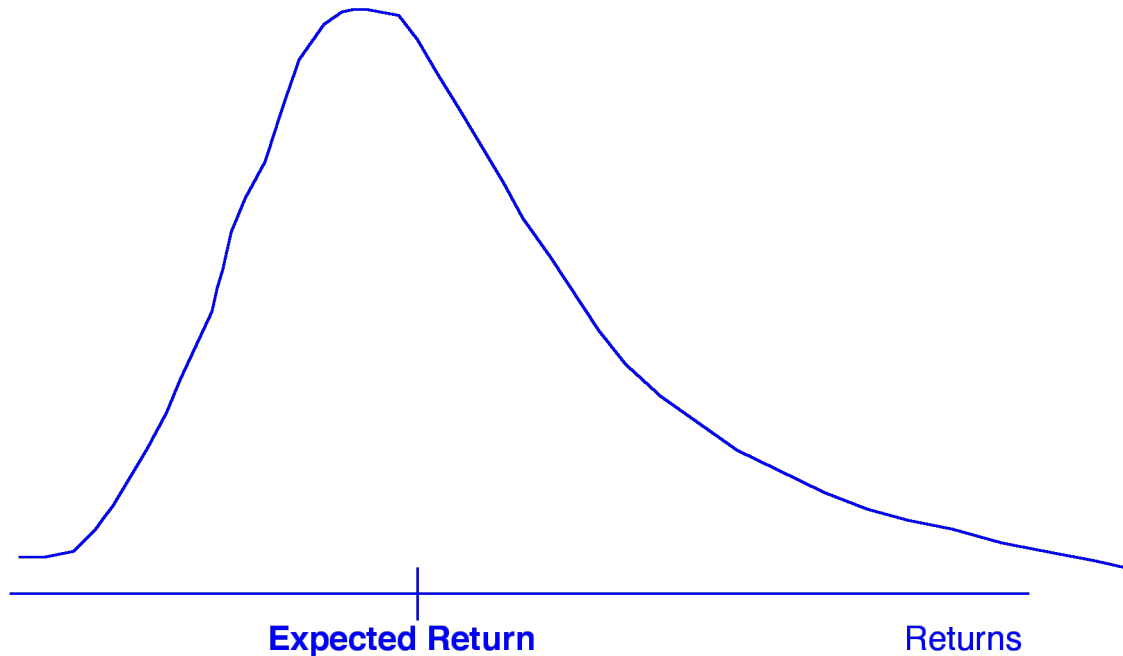
Figure 3.2: Probability Distribution for Risky Investment
