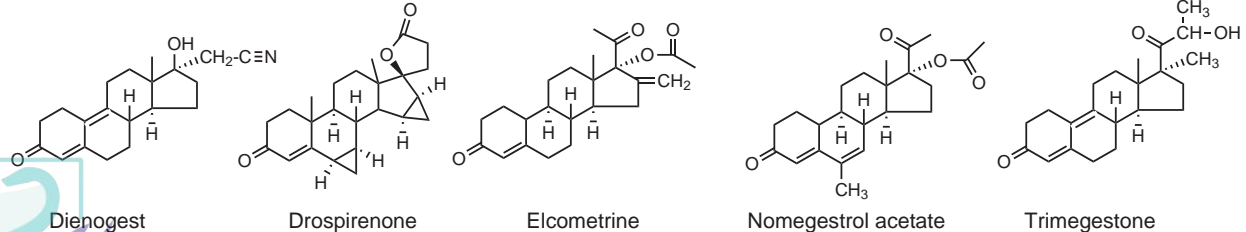
FIGURE 41.14 Progestins.
