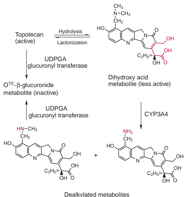
FIGURE 37.19 Topotecan metabolism.
