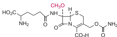
Cephamycin C
