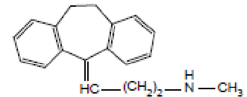
b. Nortriptyline
