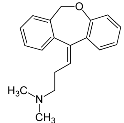
Trans Doxepin
