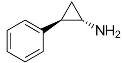
Tranylcypromine
