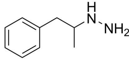
Pheniprazine
