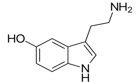
Serotonin (5HT)
