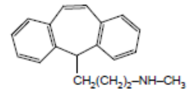
c. Protriptyline
