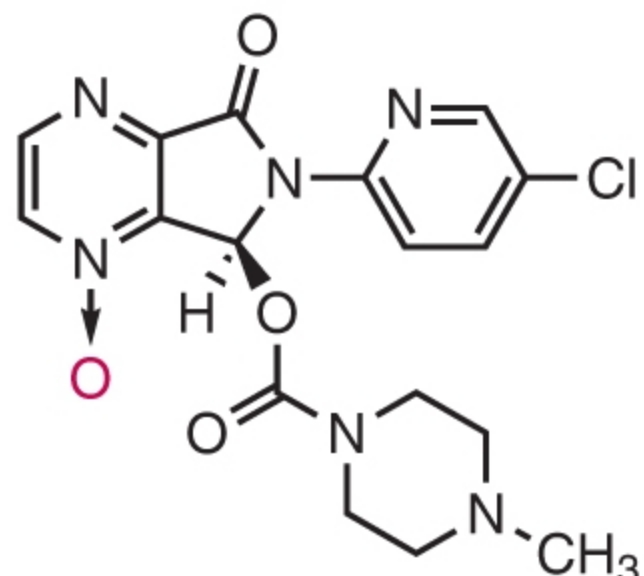
(S)-N-oxidezopiclone (inactive)
