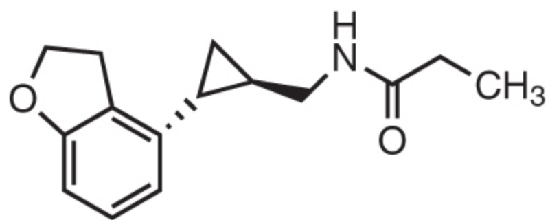
Tasimelteon
