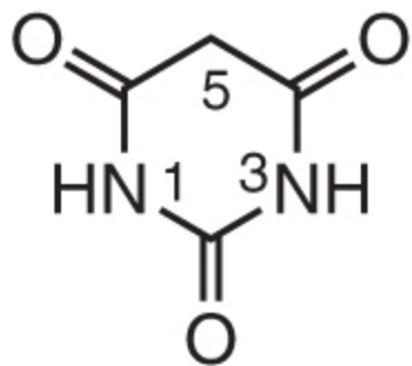
Barbituric acid
