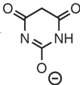
Enolate ion
