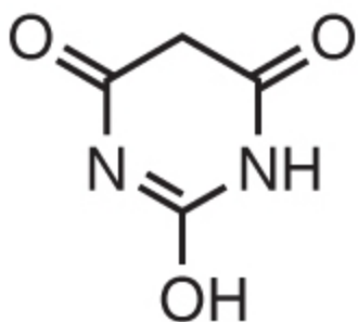
Barbituric acid
