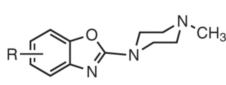
Benzoxazoles
