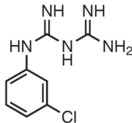
mCPBG
