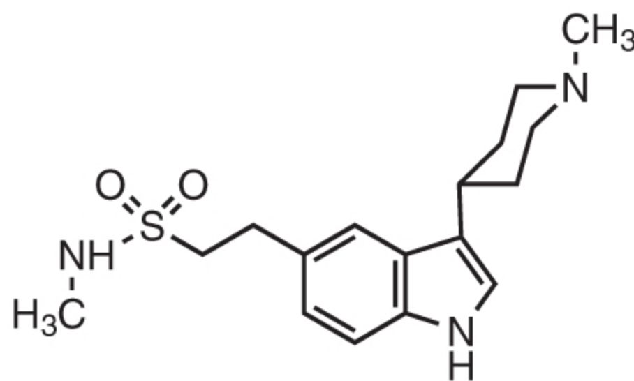
Naratriptan
