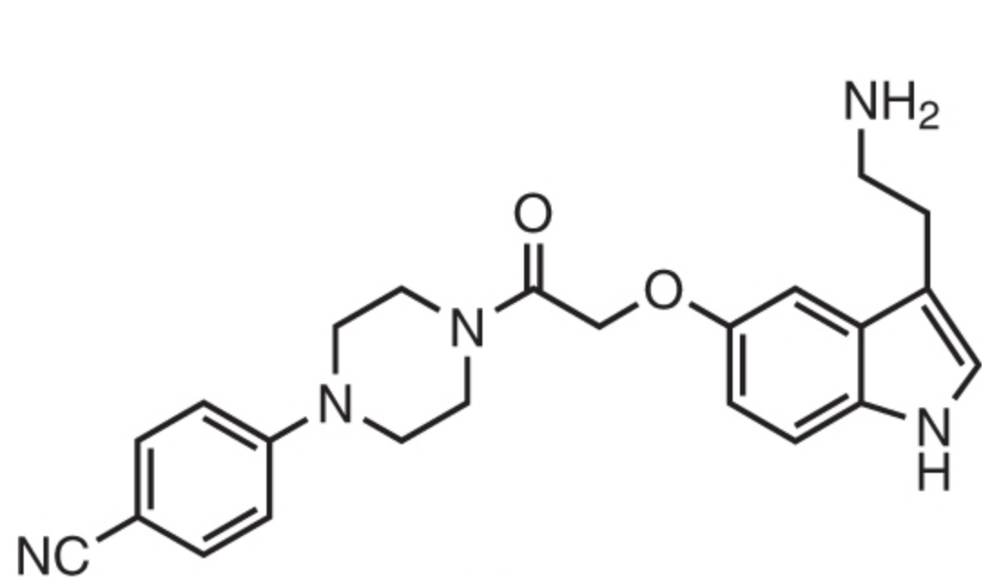
Donitriptan
