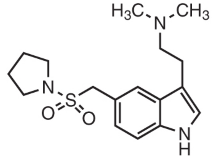
Almotriptan
