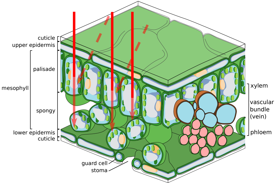
Figure 5.21. Leaf anatomy.
