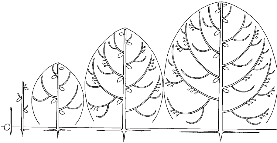
Figure 7.10. Attimis architecture model of tree growth. (From Halle et al. (1978)).
