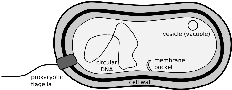
Figure 3.1. Prokaryotic cell.
