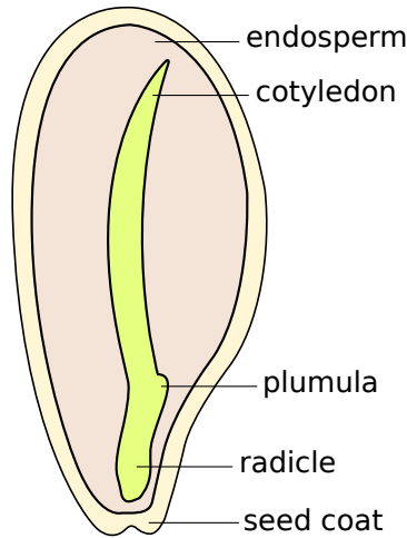
Figure 7.17. Monocot seed.
