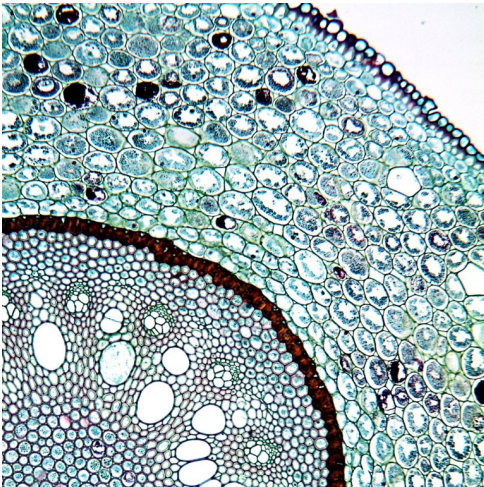
Figure 5.32. Left to right, top to bottom: Ranunculus root with 4-rayed xylem, Salix root with the lateral root developing, Smilax root with visible Casparian stripes in the endodermis; Zea root longitudinal section with root cap, division and elongation zones. Magnifications \times 100 (second) and \times 40 (others).
