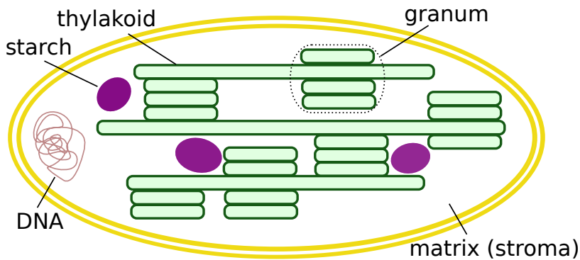
Figure 2.5. Chloroplast.
