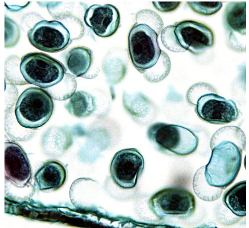
Figure 7.19. Left to right, top to bottom: Pinus (Pinopsida) microsporangia (pollen sacs), ovules sitting on seed scales, female gametophyte (endosperm 1 ) and multicellular male gametophyte (pollen). Magnifications \times 100 (first and second) and \times 400 (third and fourth).
