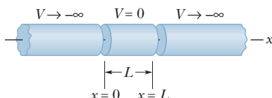
Figure 39-1 The elements of an idealized “trap” designed to confine an electron to the central cylinder. We take the semi-infinately long end cylinders to be at an infinitely great negative potential and the central cylinder to be at zero potential.
