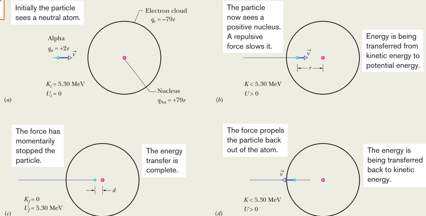
Figure 42-4 An alpha particle (a) approaches and (b) then enters a gold atom, headed toward the nucleus. The alpha particle (c) comes to a stop at the point of closest approach and (d) is propelled back out of the atom.
