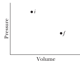
Figure 20-2 A p - V diagram showing the initial state i and the final state f of the free expansion of Fig. 20-1. The intermediate states of the gas cannot be shown because they are not equilibrium states.
