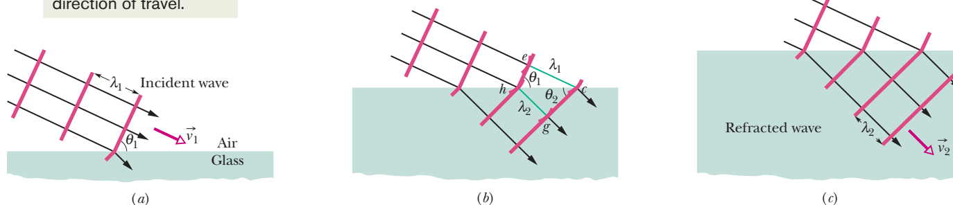
Figure 35-3 The refraction of a plane wave at an air–glass interface, as portrayed by Huygens' principle. The wavelength in glass is smaller than that in air. For simplicity, the reflected wave is not shown. Parts (a) through (c) represent three successive stages of the refraction.
