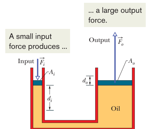
Figure 14-8 A hydraulic arrangement that can be used to magnify a force \vec{F}_i . The work done is, however, not magnified and is the same for both the input and output forces.
