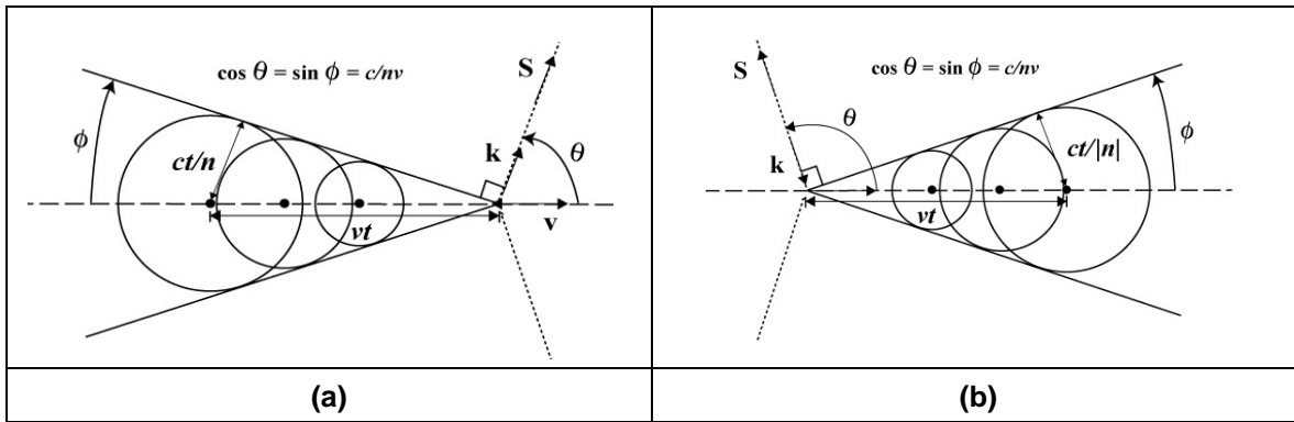
Figure 4-4. (a) Normal Cerenkov Wave and (b) Reverse Cerenkov Wave Due To Transport Through a DNM
