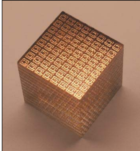
Figure 5-6. Boeing Cube Structure Designed for the Gigahertz Range
