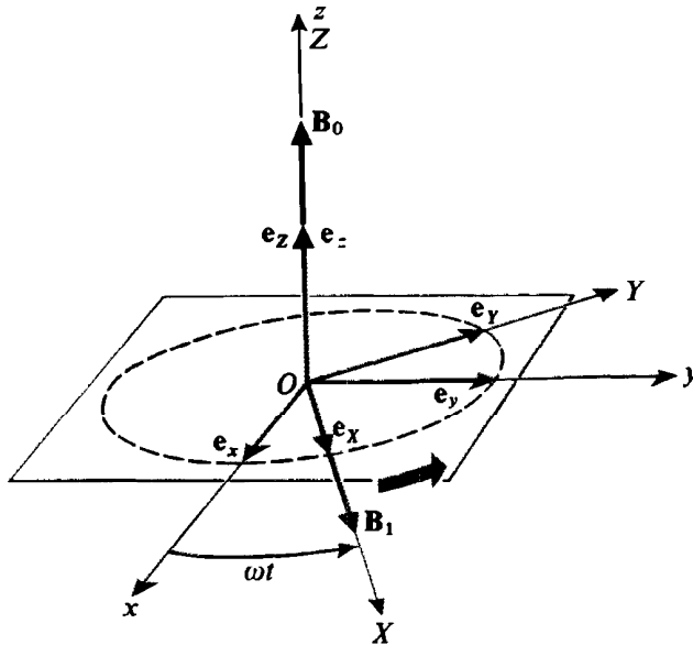
FIGURE 1 Oxyz is a fixed coordinate system. The static magnetic field \mathbf{B}_0 is directed along the Oz axis. The OXYZ system [the OX axis is the direction of the field \mathbf{B}_1(t) ] rotates about Oz with the angular velocity \omega .
