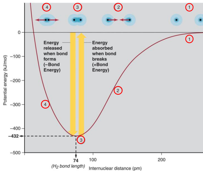
Figure 9.10 Covalent bond formation in H_2 .
