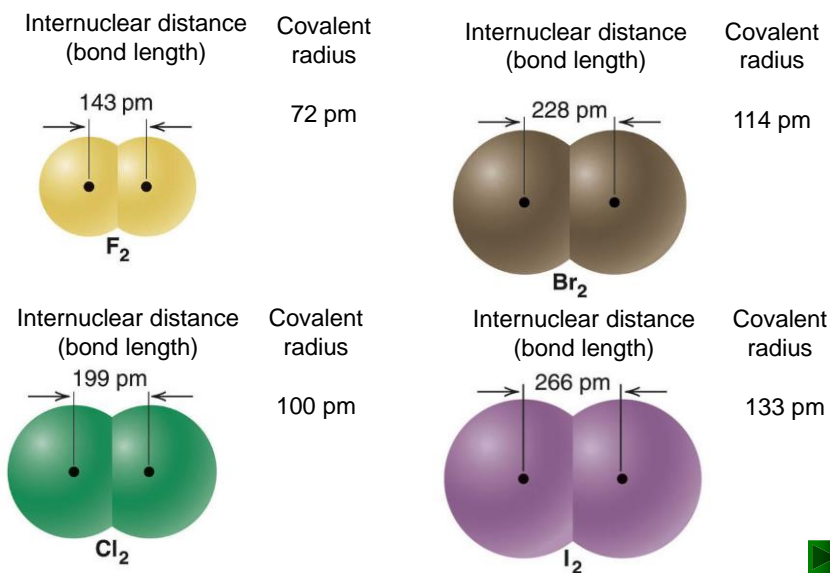
Figure 9.12 Bond length and covalent radius.
