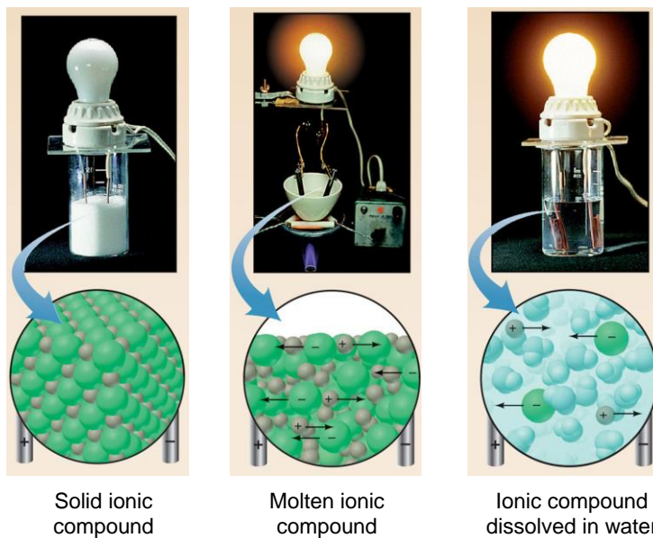
Figure 9.9 Electrical conductance and ion mobility.
