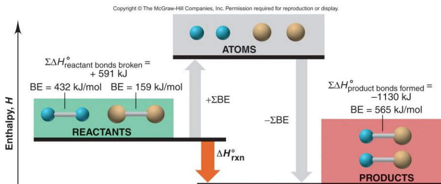
Figure 9.16 Using bond energies to calculate \Delta H^\circ_{\text{rxn}} for HF formation.
