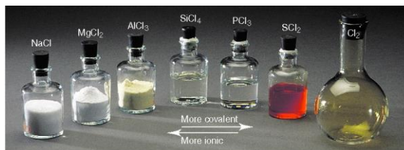
Figure 9.23 Properties of the Period 3 chlorides.
