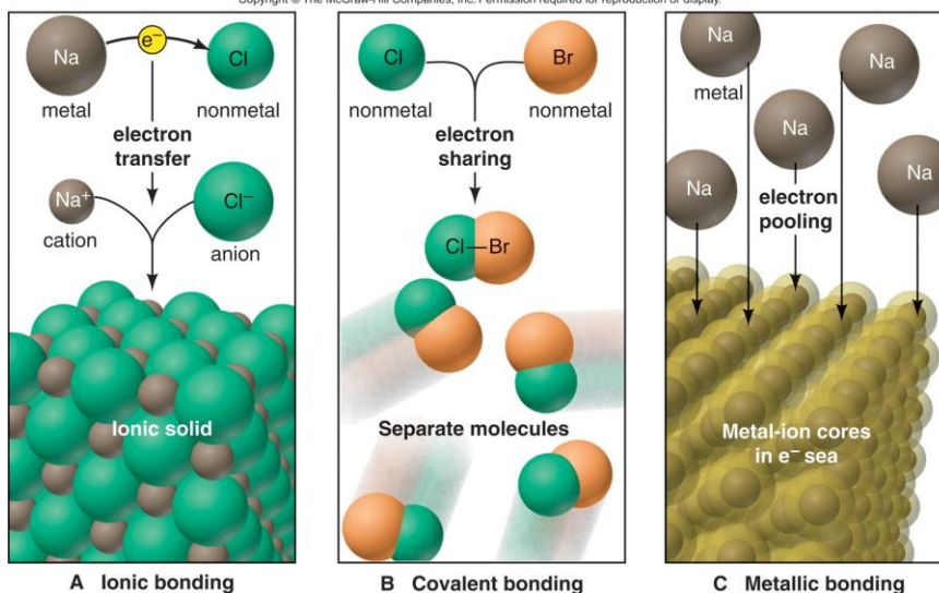
Figure 9.2 Three models of chemical bonding.
