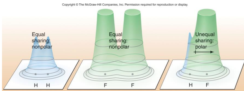
Figure 9.20 Electron density distributions in \text{H}_2 , \text{F}_2 , and HF.
