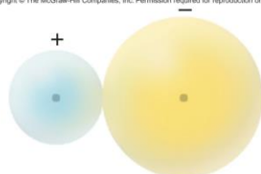
Figure 9.18 Bonding between the models.
