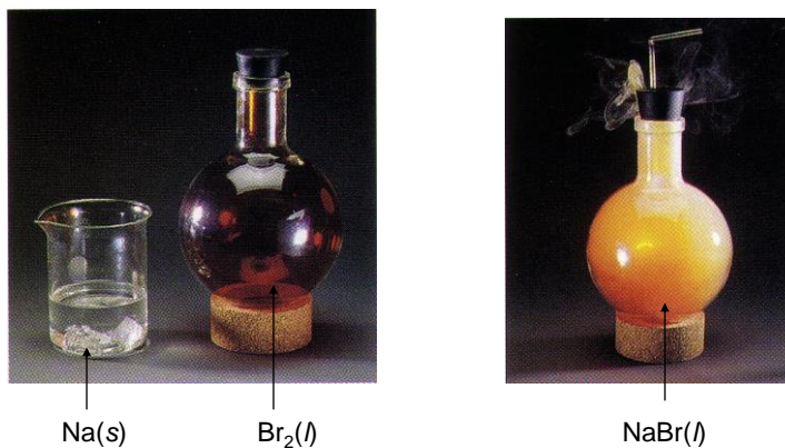
Figure 9.6 The exothermic formation of sodium bromide.
