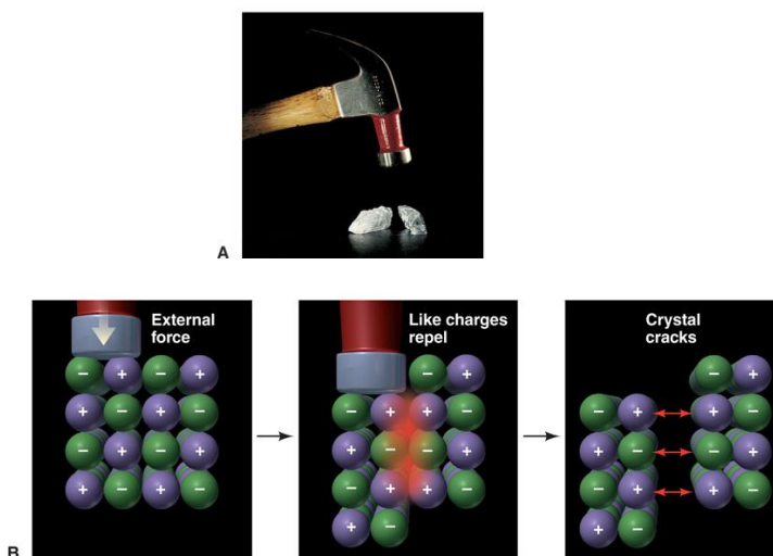
Figure 9.8 Why ionic compounds crack.
