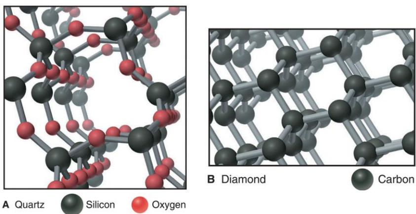
Figure 9.14 Covalent bonds of network covalent solids: quartz and diamond.
