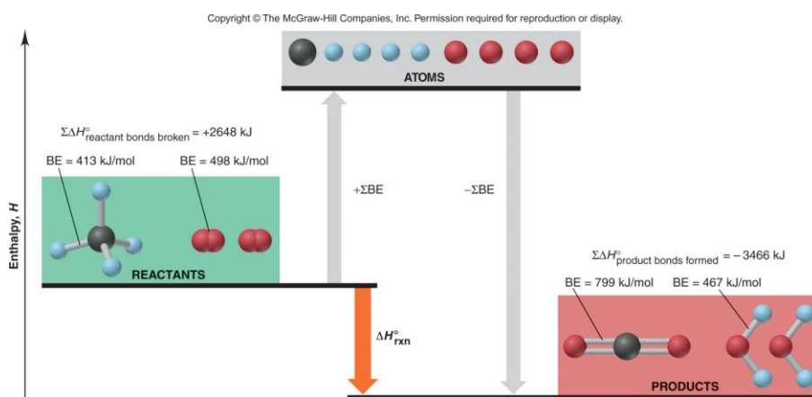
Figure 9.17 Using bond energies to calculate \Delta H^\circ_{\text{rxn}} for the combustion of methane.
