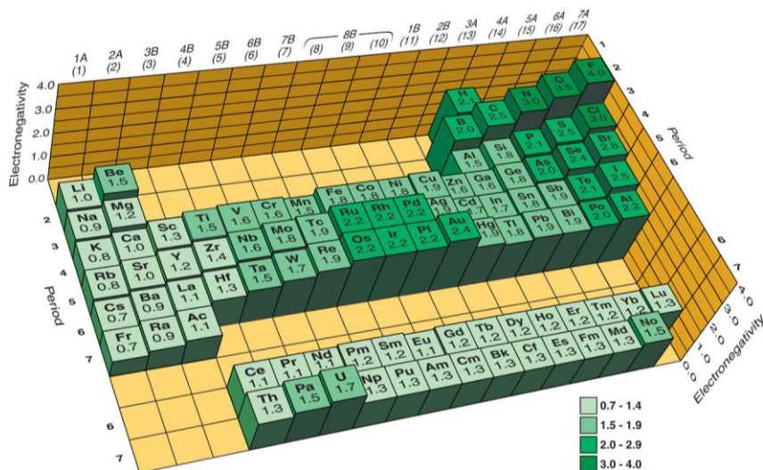
Figure 9.19 The Pauling electronegativity (EN) scale.
