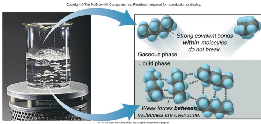
Figure 9.13 Strong forces within molecules and weak forces between them.
