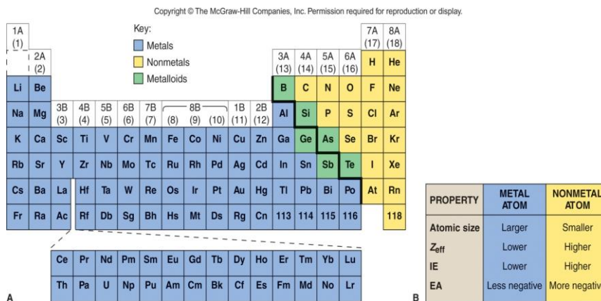
Figure 9.1 A comparison of metals and nonmetals.
