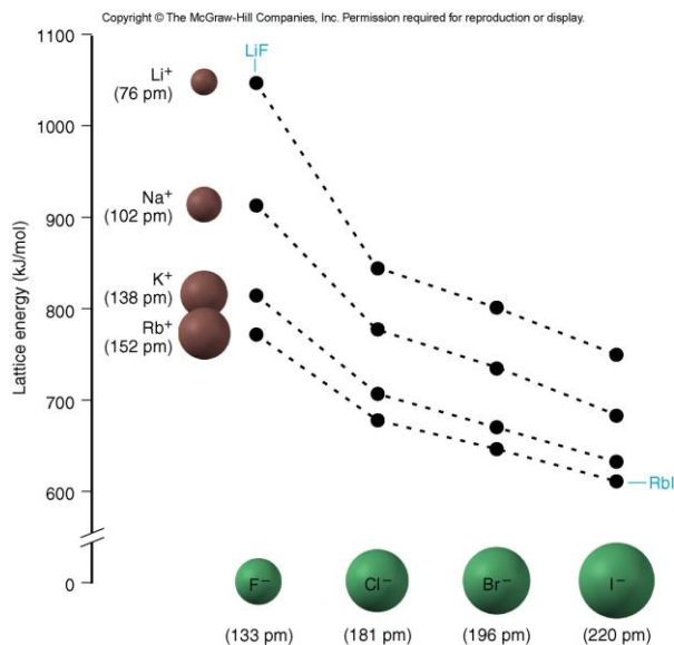
Figure 9.7 Trends in lattice energy.
