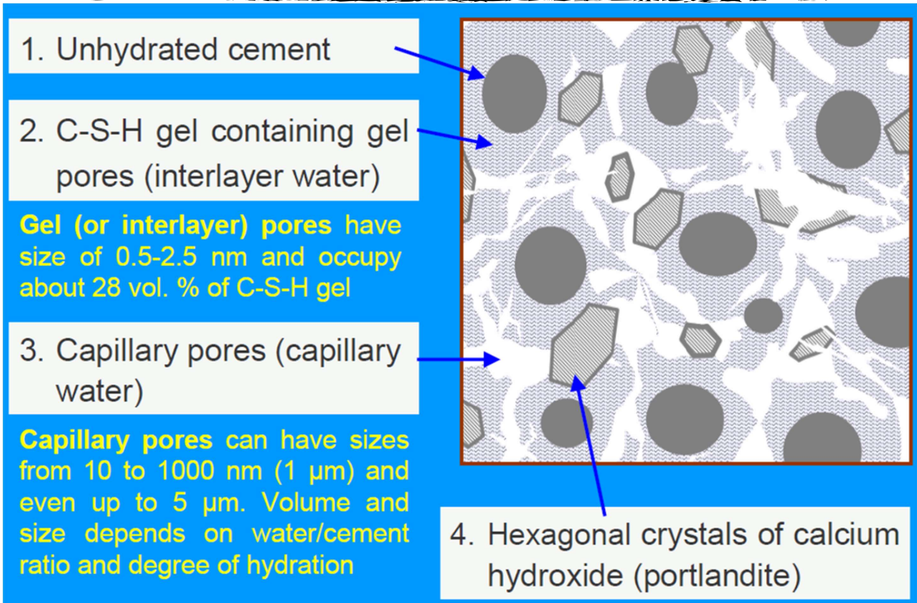
Simplified scheme of Hydrated paste microstructure
