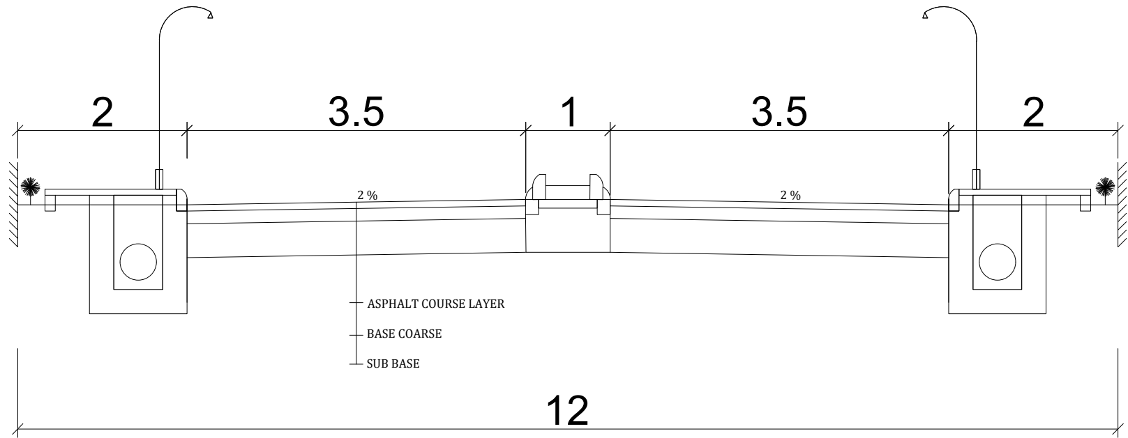
TYPICAL CROSS SECTION Scale 1:200
