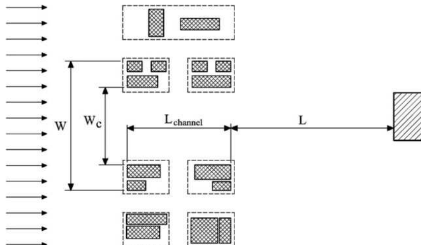
FIGURE C6.8-1 Flow Amplification for Channelized Conditions
