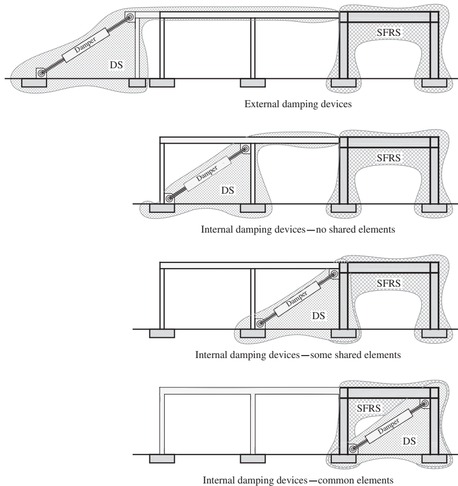
FIGURE C18.1-1 Damping System (DS) and Seismic Force-Resisting System (SFERS) Configurations
