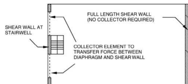
FIGURE 12.10-1 Collectors
