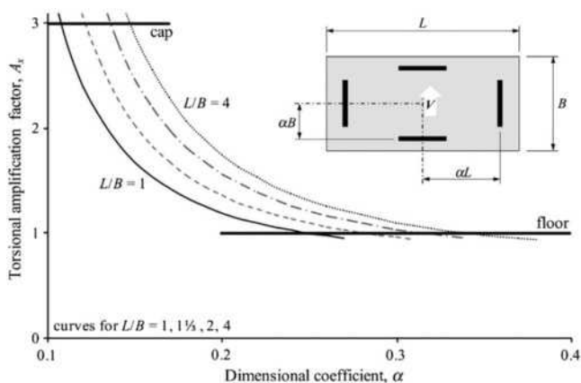
FIGURE C12.8-5 Torsional Amplification Factor for Symmetric Rectangular Buildings
