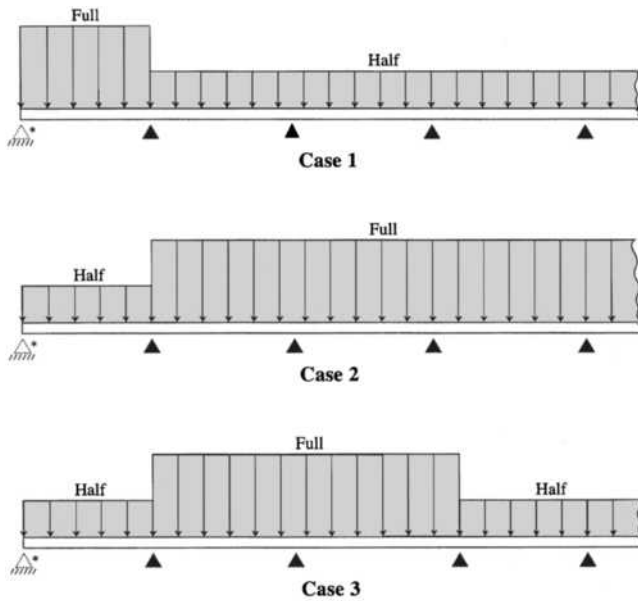
FIGURE 7.5-1 Partial Loading Diagrams for Continuous Beams
