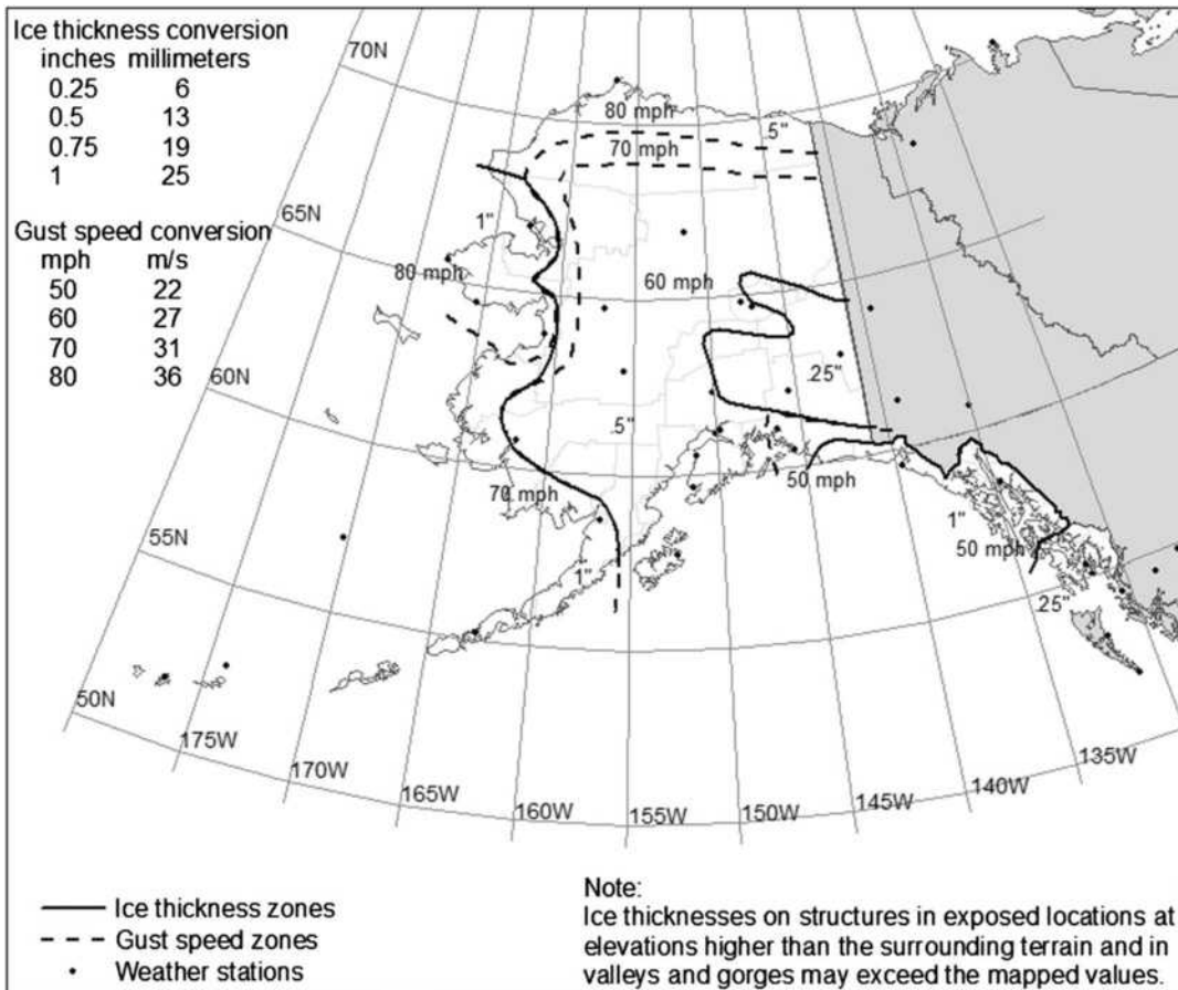
FIGURE 10.4-6 500-Year Mean Recurrence Interval Uniform Ice Thicknesses Caused by Freezing Rain with Concurrent 3-Second Gust Speeds: Alaska
