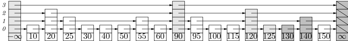
Figure 9.12: The skip list from Figure 9.11, showing a possible representation. The data structure is an ordered list whose nodes contain random numbers of pointers to later nodes (which allow intervening items in the list to be skipped during a search; hence the name). If a node has at least k pointers, then it contains a pointer to the next node that has at least k pointers. A node for \infty at the right allows us to avoid tests for null. Again, the nodes looked at during a search for 127 are shaded; the darker shading indicates nodes that limit the search.
