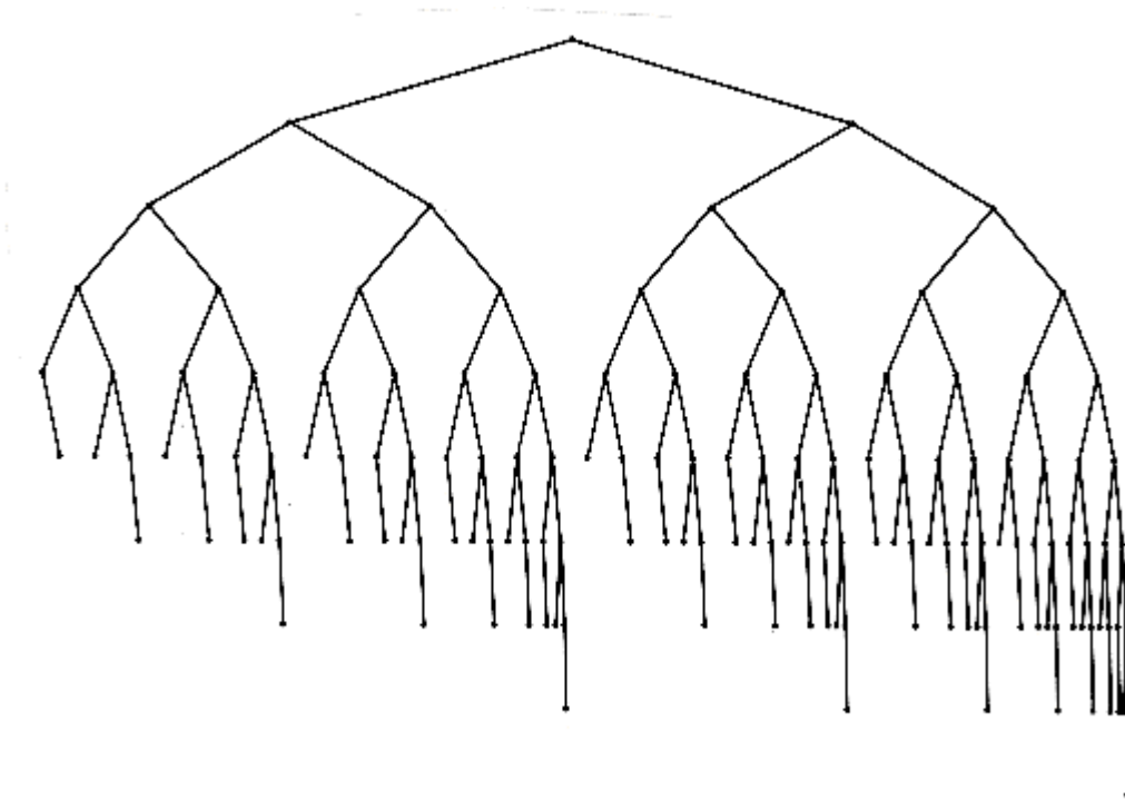
Figure 4.30 Smallest AVL tree of height 9
