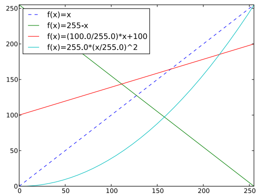
Figure 1.4: Example graylevel transforms. Three example functions together with the identity transform showed as a dashed line.
