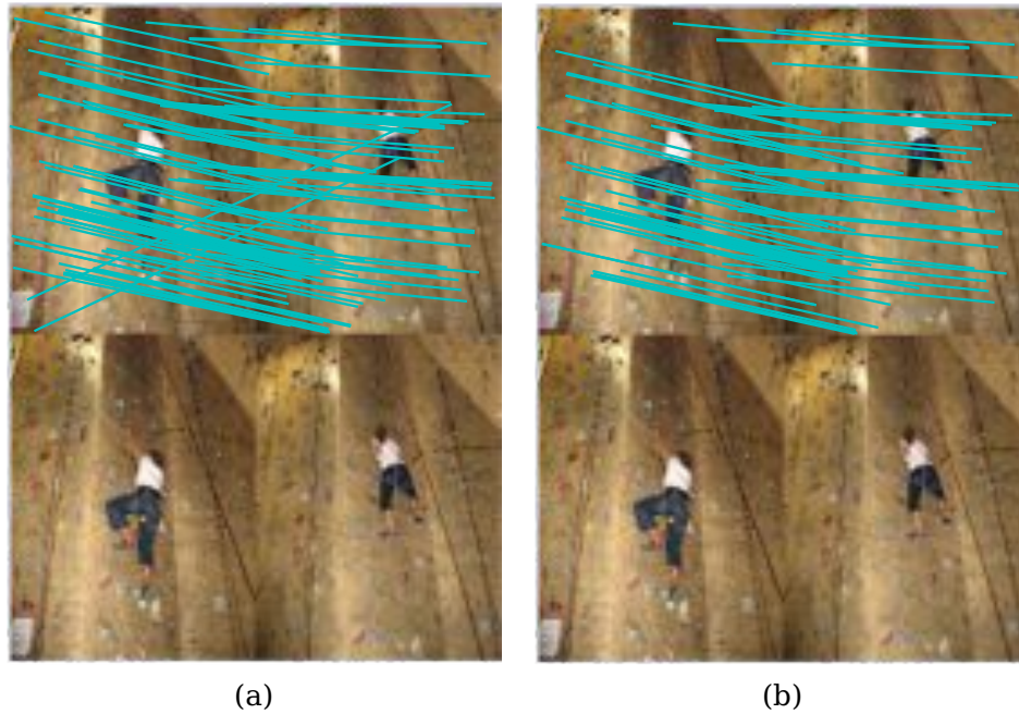
Figure 2.7: An example of matching SIFT features between two images. (a) matches from features in the left image without using the two-sided match function (b) the remaining matches after using the two-sided version.
