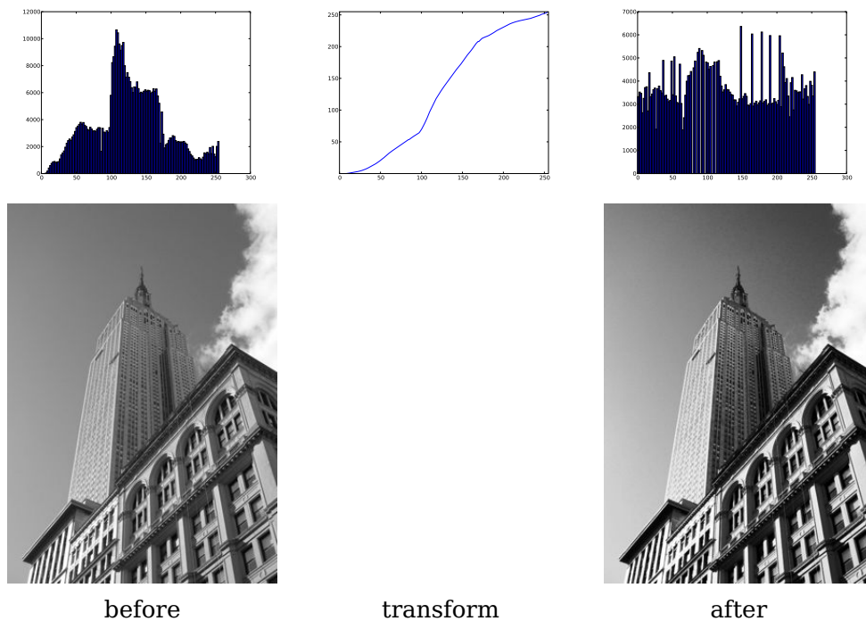
Figure 1.6: Example of histogram equalization. On the left is the original image and histogram. The middle plot is the graylevel transform function. On the right is the image and histogram after histogram equalization.
