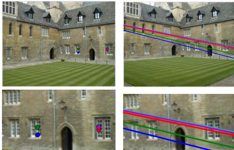
Figure 5.4: Epipolar lines in view 1 shown for five points in view 2 of the Merton1 data. The bottom row shows a close up of the area around the points. The lines can be seen to converge on a point outside the image to the left. The lines show where point correspondences can be found in the other image (the color coding matches between lines and points).
