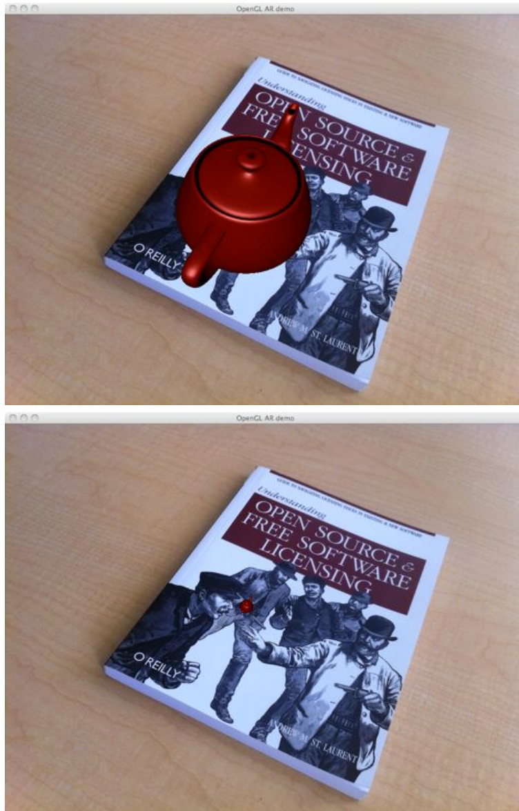
Figure 4.5: Augmented reality. Placing a computer graphics model on a book in a scene using camera parameters computed from feature matches. (top) the Utah teapot rendered in place aligned with the coordinate axis. (bottom) sanity check to see the position of the origin.
