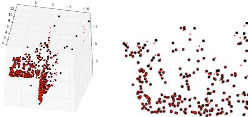
Figure 5.5: Triangulated points using camera matrices and point correspondences. The estimated points are shown with black circles and the true points with red dots. (left) view from above and to the side. (right) close up of the points from one of the building walls.
