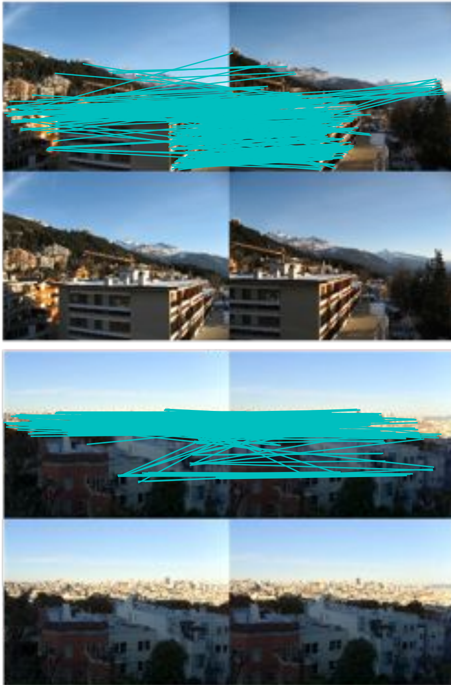
Figure 2.2: Example of matches resulting from applying normalized cross correlation to patches around Harris corner points.
