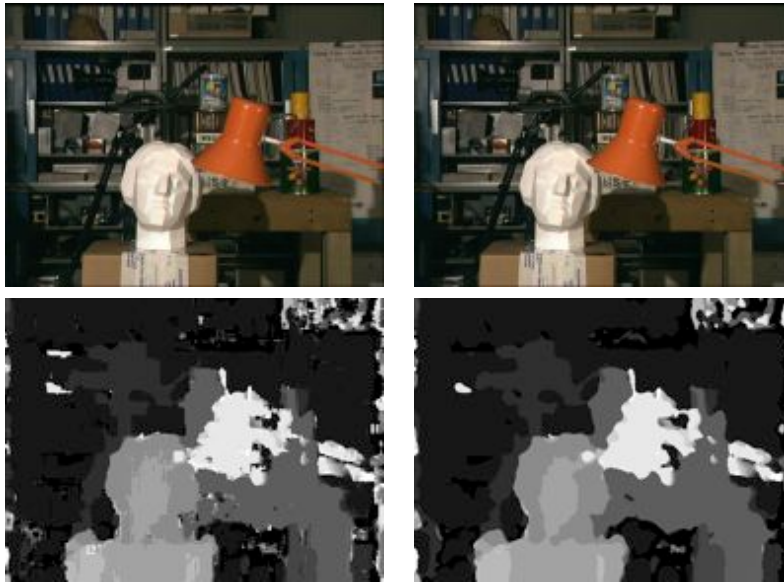
Figure 5.10: Example of computing disparity maps from a stereo image pair with normalized cross-correlation.
