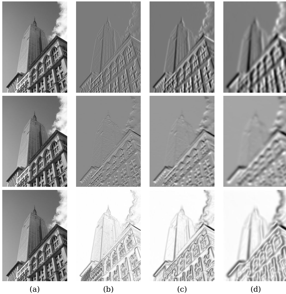
Figure 1.11: An example of computing image derivatives using Gaussian derivatives. (top) x-derivative, (middle) y-derivative and (bottom) gradient magnitude. (a) original image in grayscale, (b) Gaussian derivative filter with \sigma = 2 , (c) with \sigma = 5 , (d) with \sigma = 10 .
