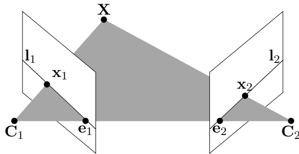
Figure 5.1: An illustration of epipolar geometry. A 3D point X is projected to x_1 and x_2 , in the two views respectively. The baseline between the two camera centers, C_1 and C_2 , intersect the image planes in the epipoles, e_1 and e_2 . The lines l_1 and l_2 are called epipolar lines.
