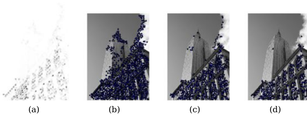
Figure 2.1: An example of corner detection with the Harris corner detector. (a) the Harris response function, (b), (c) and (d) corners detected with threshold 0.01, 0.05, and 0.1 respectively.
