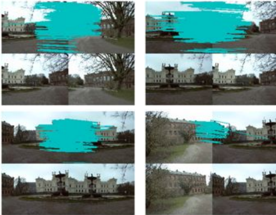
Figure 3.11: Matching correspondences found between consecutive image pairs using SIFT features.
