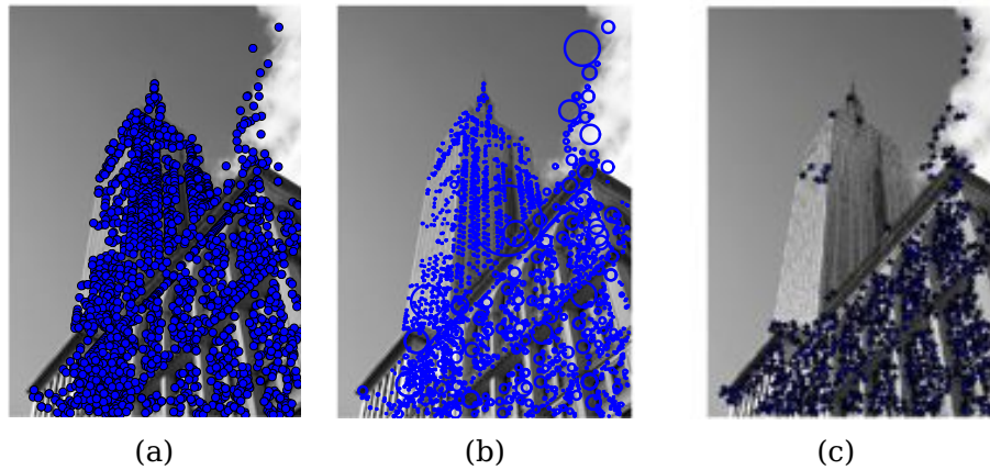
Figure 2.4: An example of extracting SIFT features for an image. (a) SIFT features (b) SIFT features shown with circle indicating the scale of the feature (c) Harris points for the same image for comparison.
