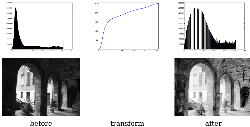
Figure 1.7: Example of histogram equalization. On the left is the original image and histogram. The middle plot is the graylevel transform function. On the right is the image and histogram after histogram equalization.
