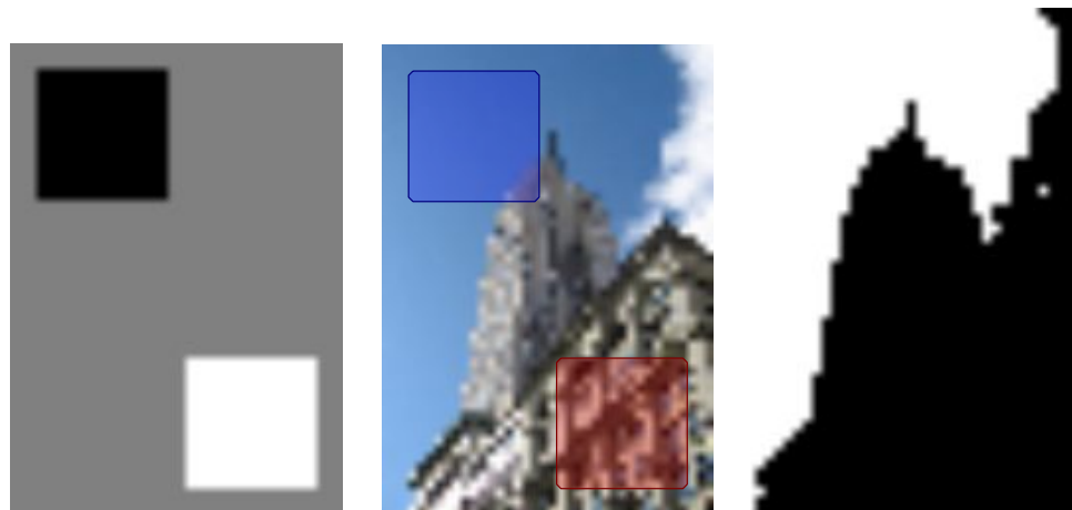
Figure 9.2: An example of graph cut segmentation using a Bayesian probability model. Image is downsampled to size 54 \times 38 . (left) label image for model training. (center) training regions shown on the image. (right) segmentation.
