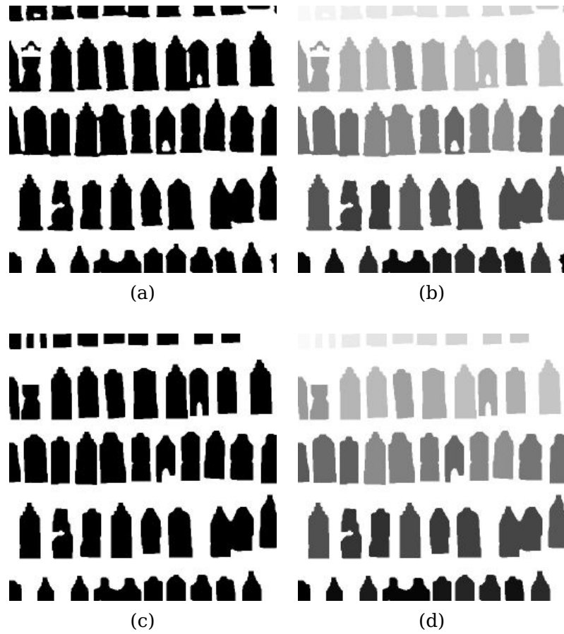
Figure 1.12: An example of morphology. Binary opening to separate objects followed by counting them. (a) original binary image, (b) label image corresponding to the original, grayvalues indicate object index, (c) binary image after opening, (d) label image corresponding to the opened image.
