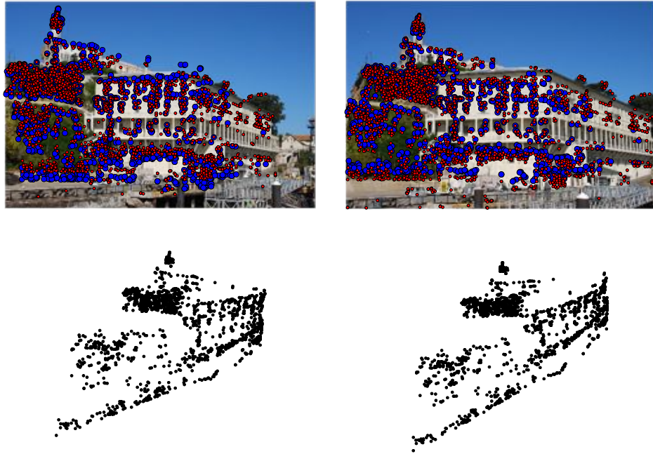
Figure 5.8: Example of computing a 3D reconstruction from a pair of images using image matches. (top) the two images with feature points shown in red and reprojected reconstructed 3D points shown in blue. (bottom) the 3D reconstruction.
