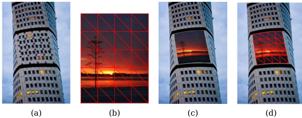
Figure 3.5: An example of piecewise affine warping using Delaunay triangulated landmark points. (a) the target image with landmarks. (b) image with triangulation. (c) with warped image. (d) with warped image and triangulation.
