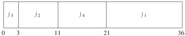
Figure 10.3 Schedule #2 (optimal)
