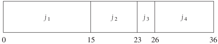
Figure 10.2 Schedule #1
