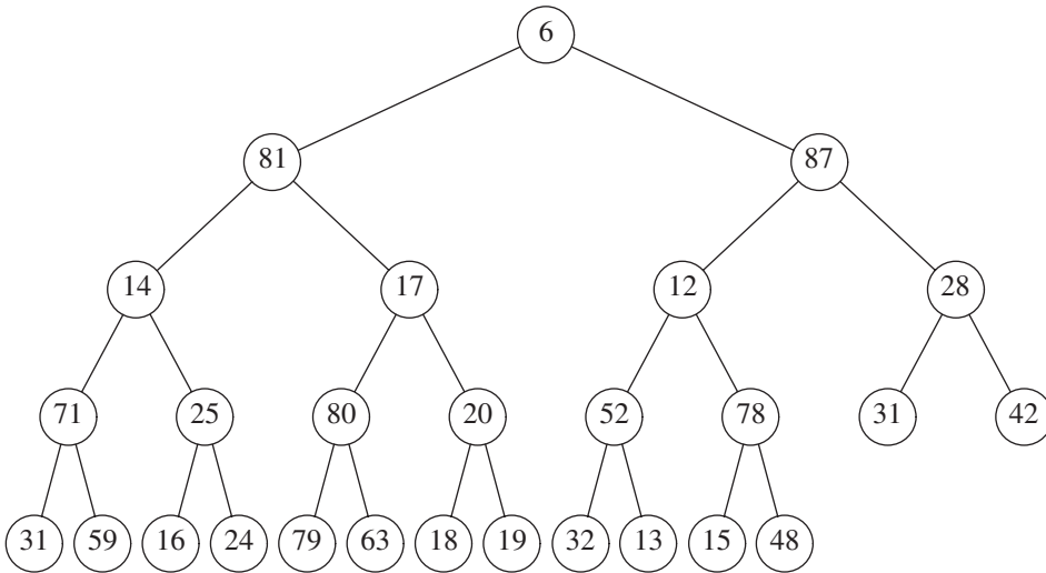
Figure 6.57 Min-max heap
