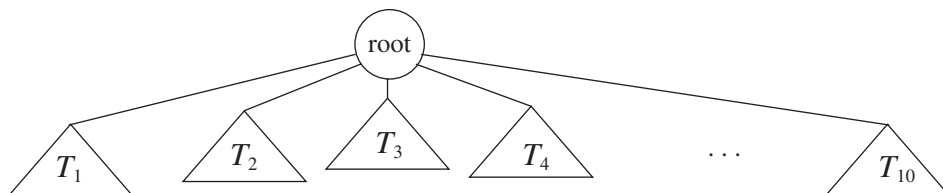
Figure 4.1 Generic tree
