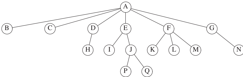
Figure 4.2 A tree
