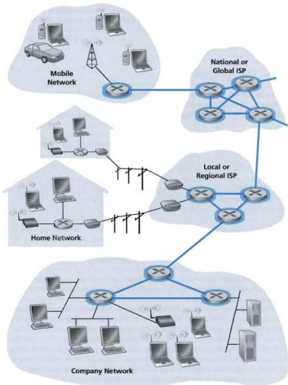
Figure 1.11 ♦ The network core
