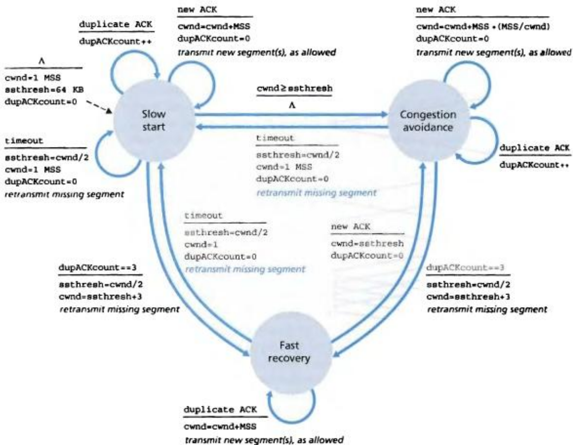
Figure 3.52 ♦ FSM description of TCP congestion control
