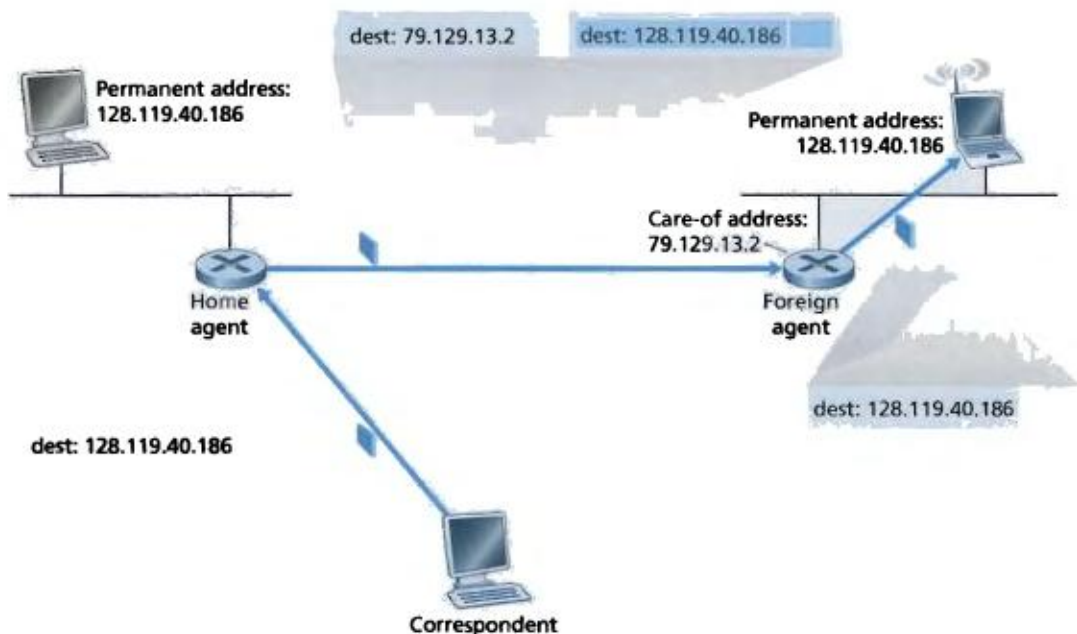
Figure 6.24 ♦ Encapsulation and decapsulation
