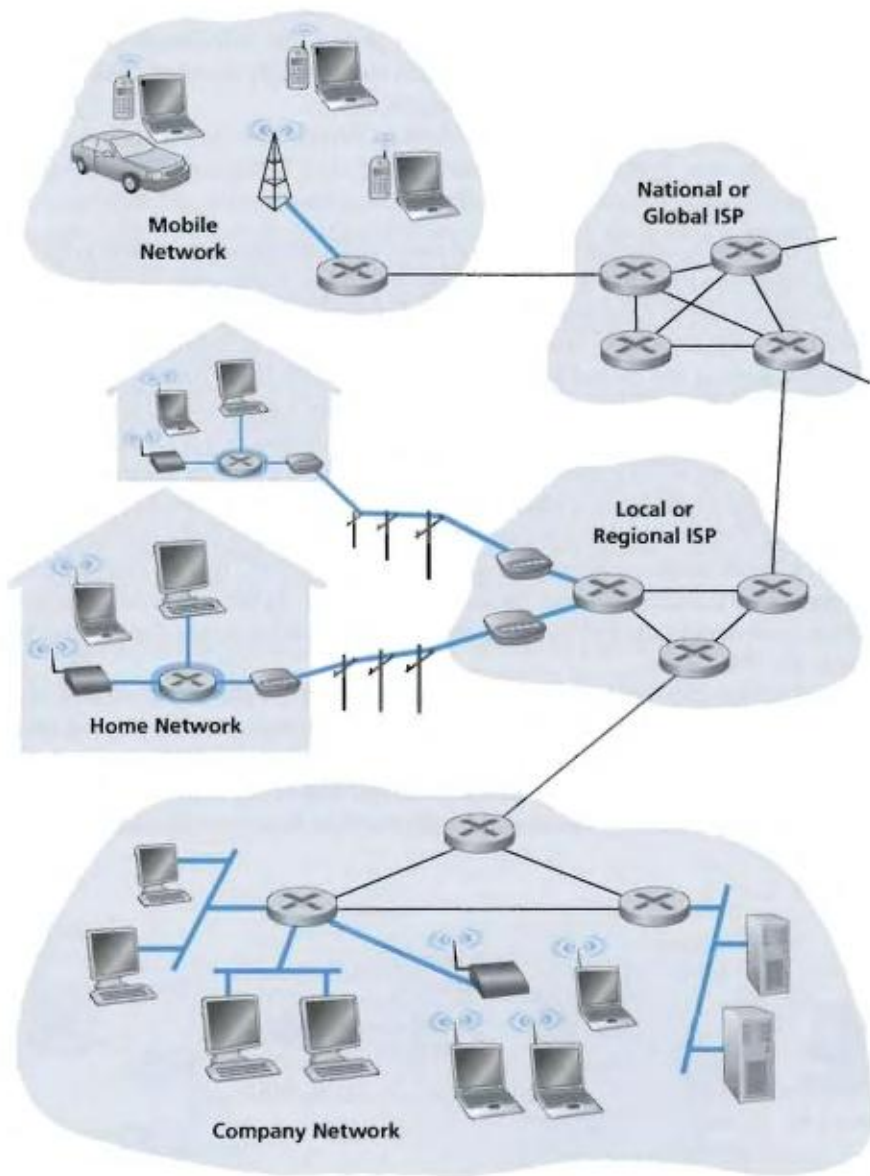
Figure 1.4 ♦ Access networks
