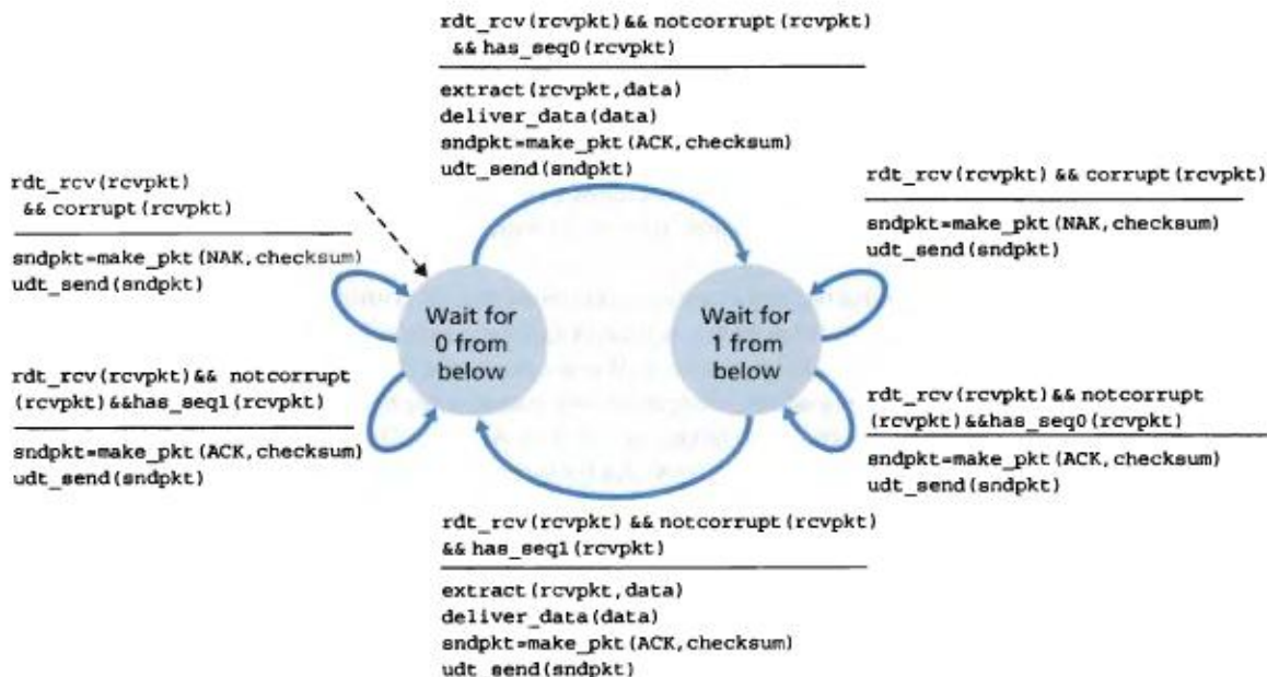
Figure 3.12 ♦ rdt2.1 receiver
