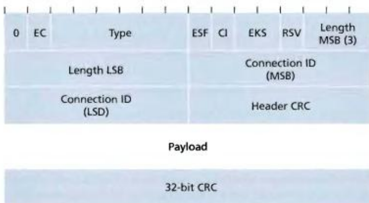
Figure 6.18 ♦ 802.16 packet
