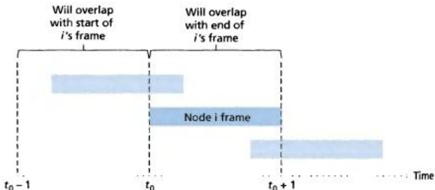
Figure 5.12 ♦ Interfering transmissions in pure ALOHA
