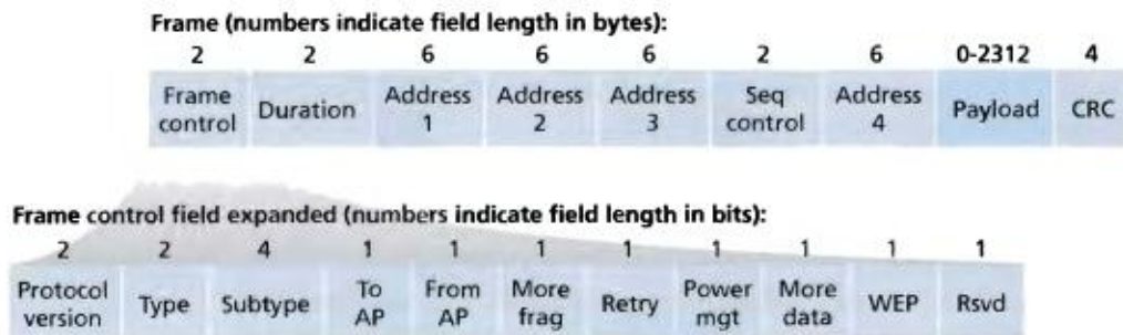
Figure 6.13 ♦ The 802.11 frame
