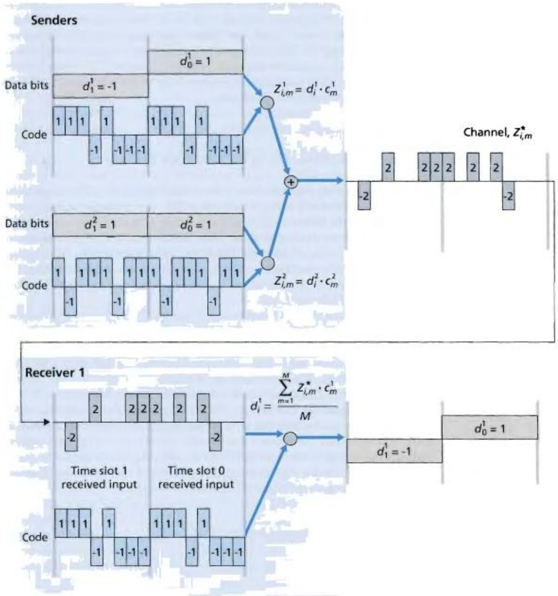
Figure 6.6 ♦ A two-sender CDMA example
