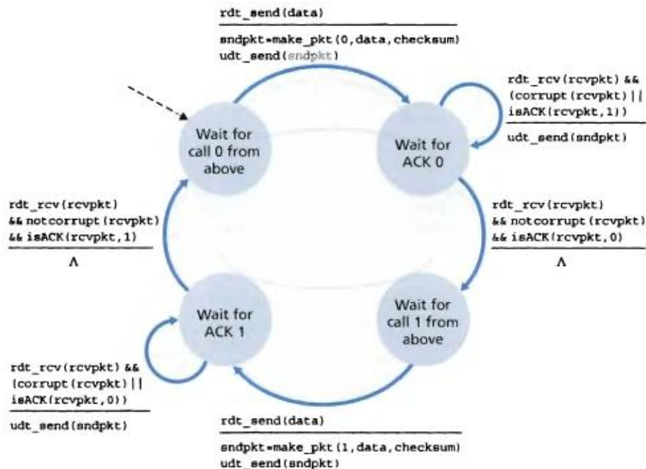
Figure 3.13 ♦ rdt2.2 sender
