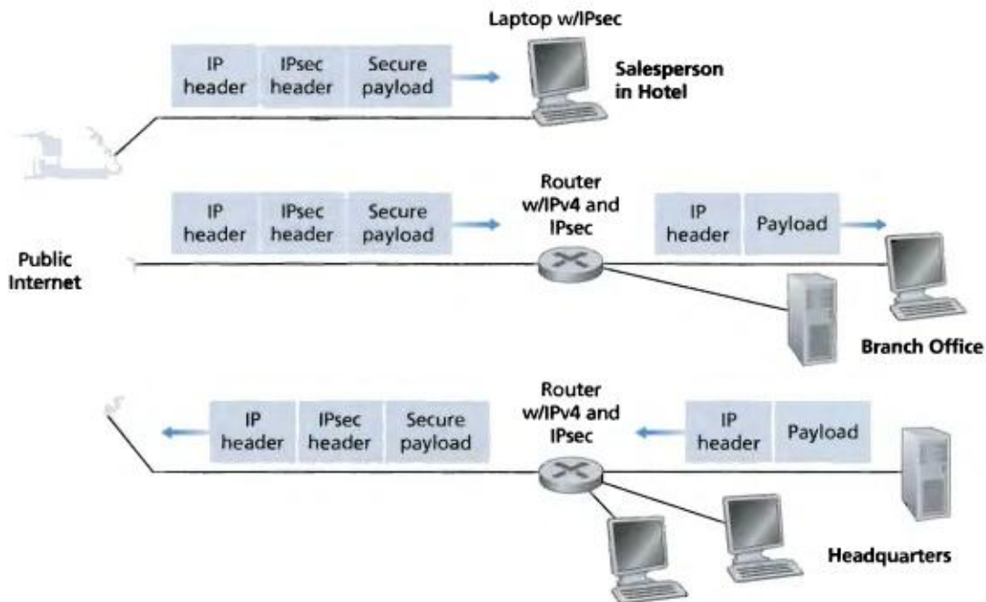
Figure 8.28 ♦ Virtual Private Network (VPN)
