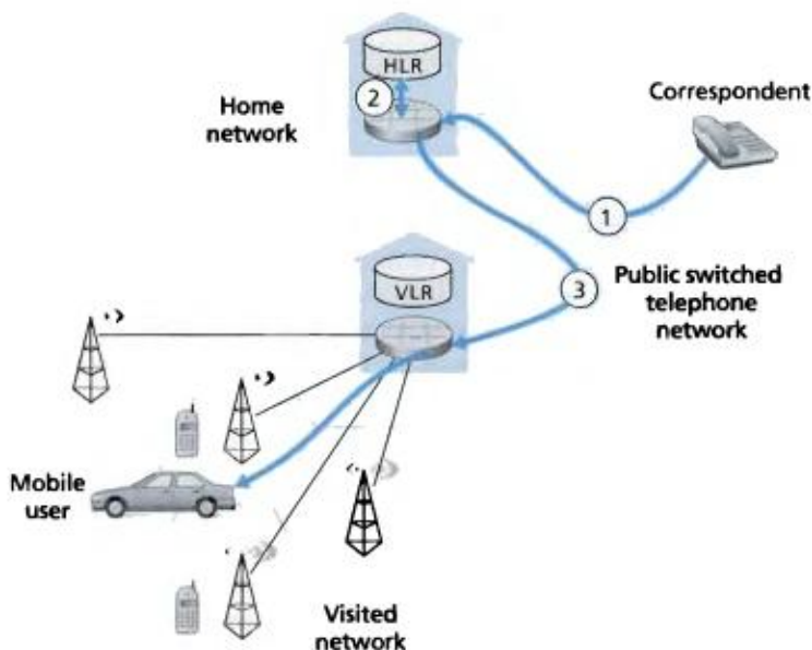
Figure 6.29 ♦ Placing a call to a mobile user: indirect routing
