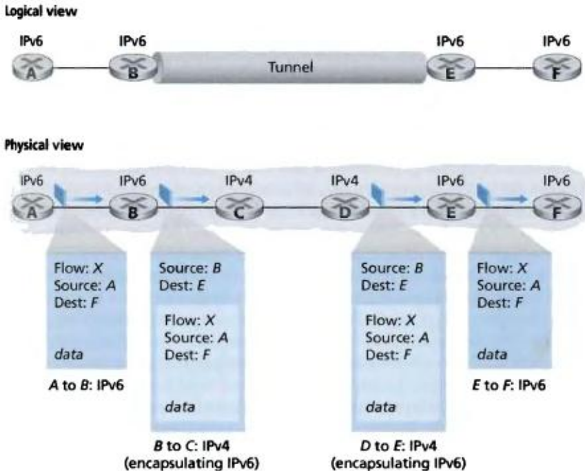
Figure 4.26 • Tunneling
