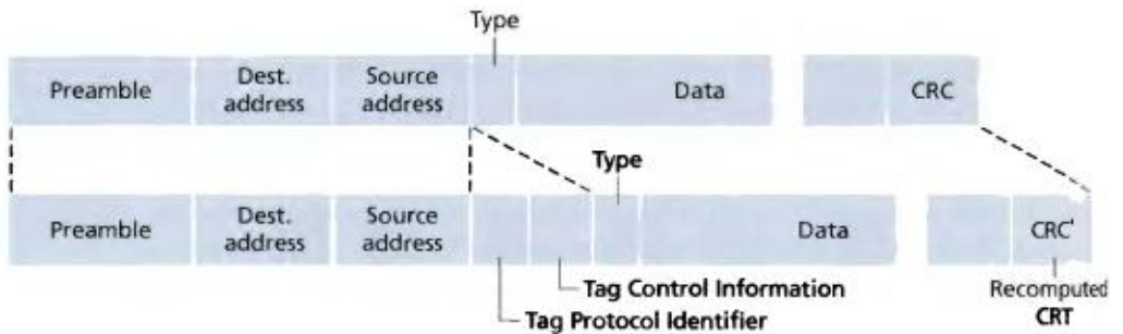
Figure 5.32 ♦ Original Ethernet frame (top), 802.1Q-tagged Ethernet VLAN frame (below)
