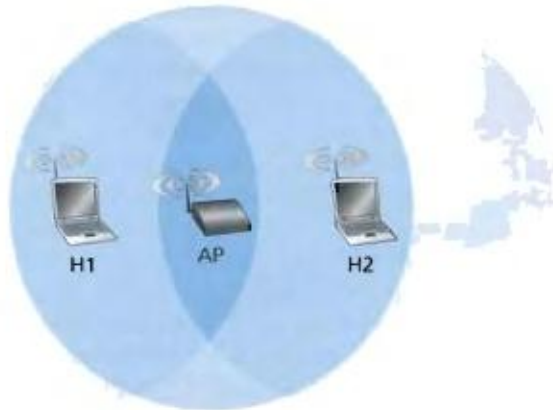
Figure 6.11 ♦ Hidden terminal example: H1 is hidden from H2, and vice versa.
