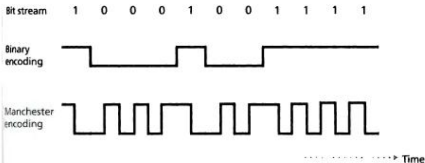
Figure 5.23 ♦ Manchester encoding
