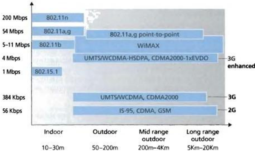
Figure 6.2 ♦ Link characteristics of selected wireless network standards
