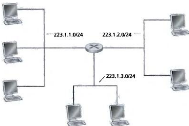
Figure 4.16 ♦ Subnet addresses
