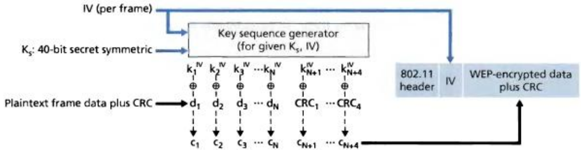
Figure 8.31 ♦ 802.11 WEP protocol
