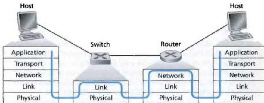
Figure 5.29 ♦ Packet processing in switches, routers, and hosts
