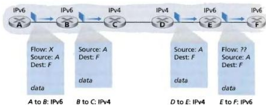
Figure 4.25 ♦ A dual-stack approach
