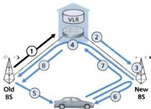
Figure 6.31 ♦ Steps in accomplishing a handoff between base stations with a common MSC
