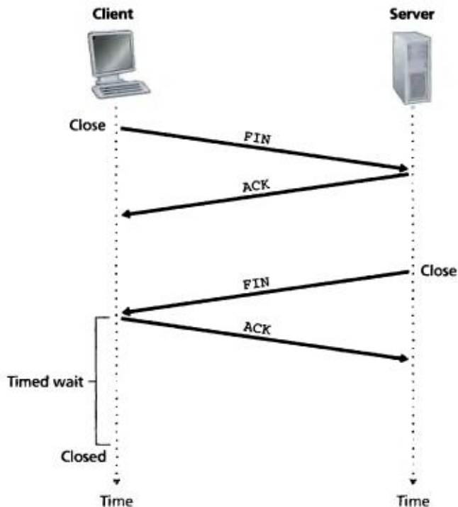
Figure 3.40 ♦ Closing a TCP connection
