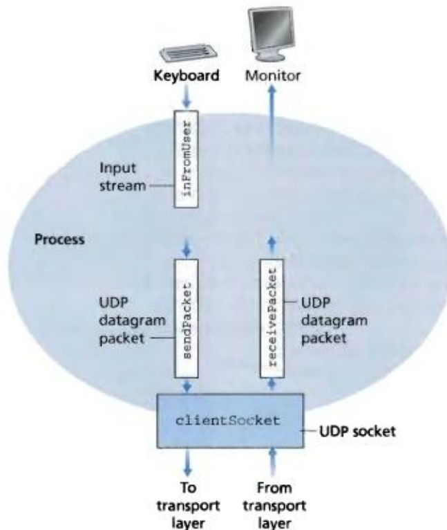
Figure 2.33 ♦ UDPCliient has one stream; the socket accepts packets from the process and delivers packets to the process.
