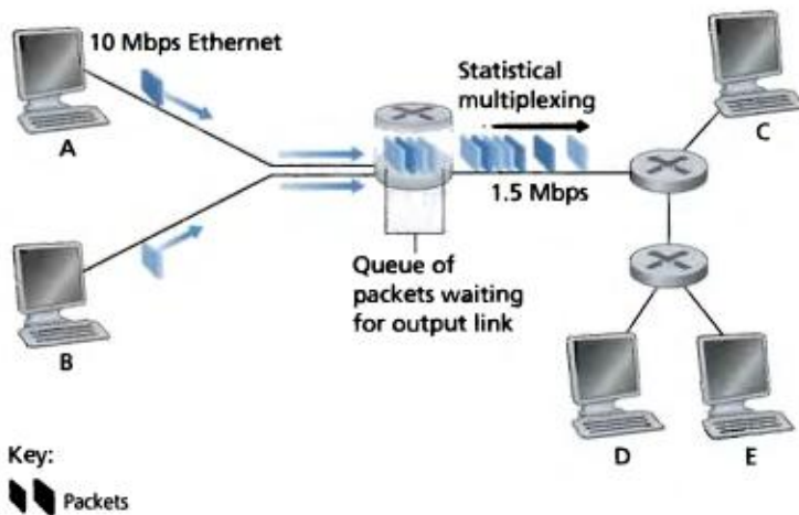
Figure 1.14 ♦ Packet switching
