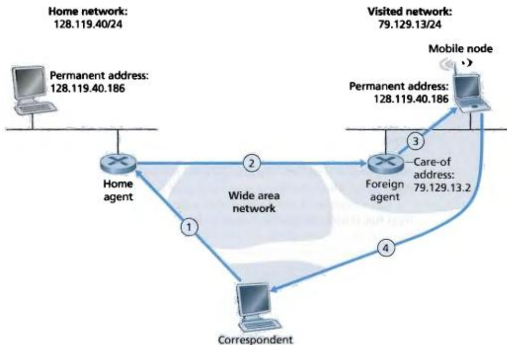
Figure 6.23 ♦ Indirect routing to a mobile node
