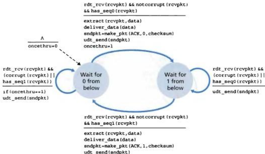
Figure 3.14 ♦ rdt2.2 receiver
