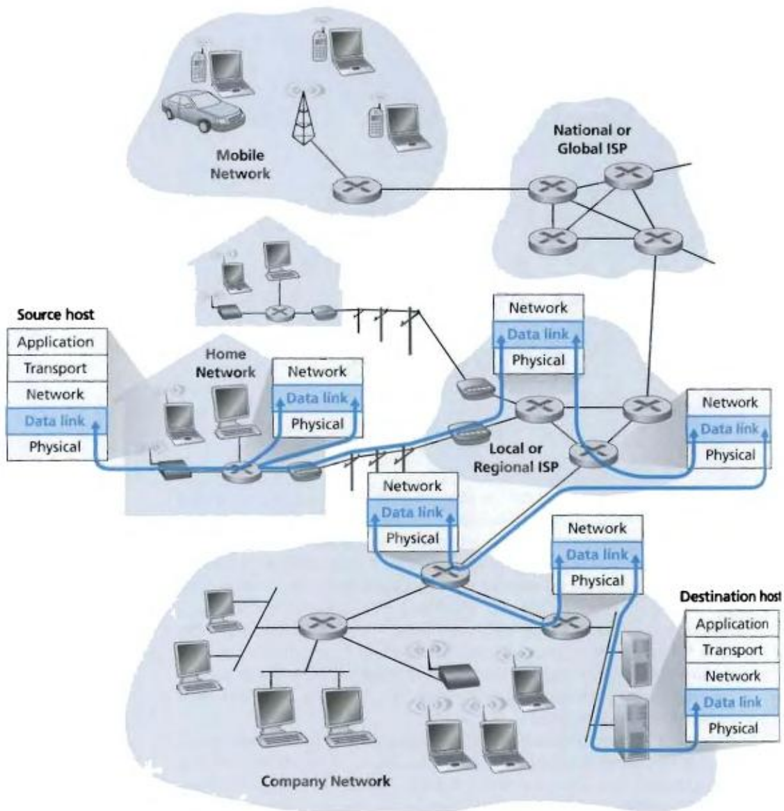
Figure 5.1 ♦ The link layer
