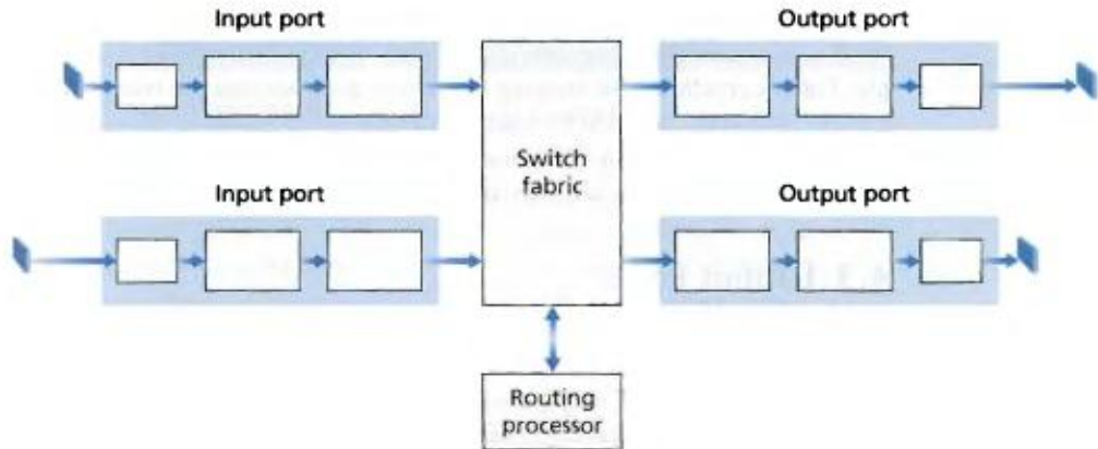
Figure 4.6 ♦ Router architecture
