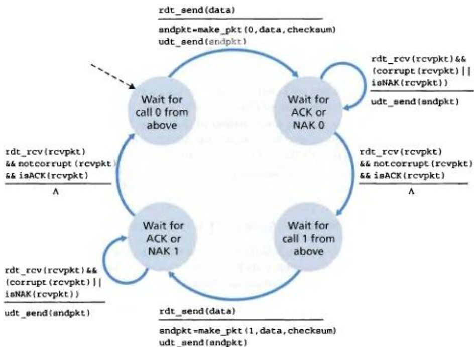
Figure 3.11 ♦ rdt2.1 sender
