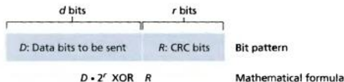
Figure 5.7 ♦ CRC
