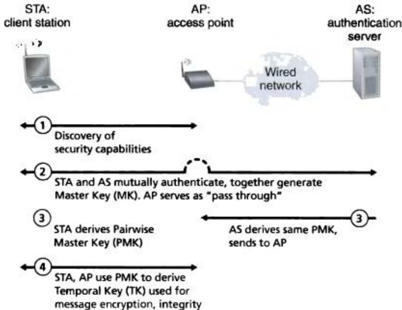
Figure 8.32 ♦ 802.11i: four phases of operation
