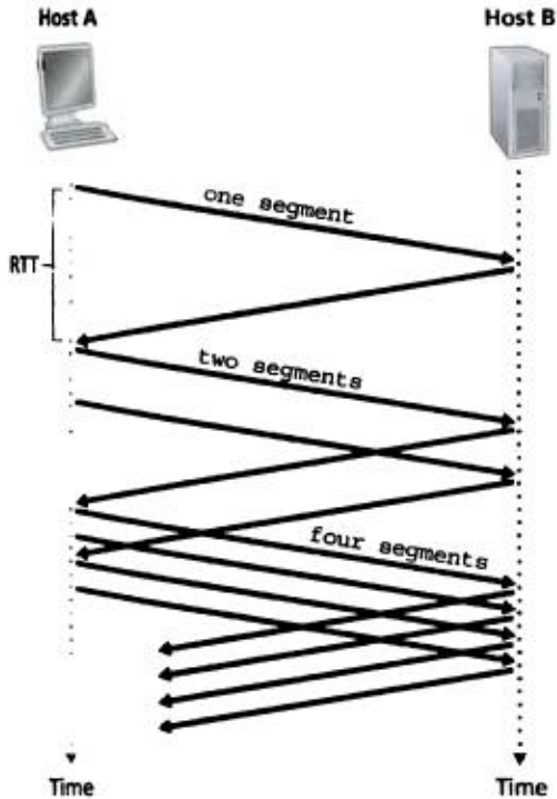
Figure 3.51 ♦ TCP slow start
