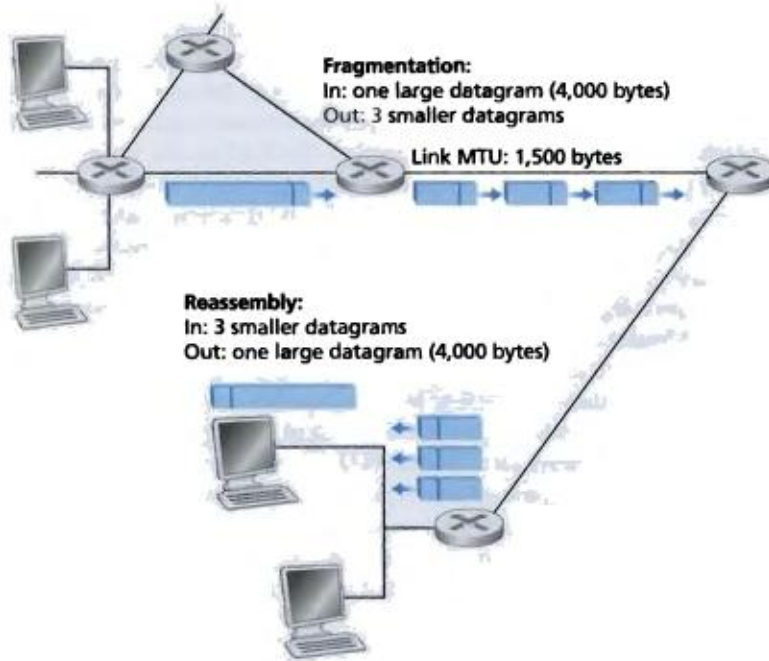
Figure 4.14 ♦ IP fragmentation and reassembly
