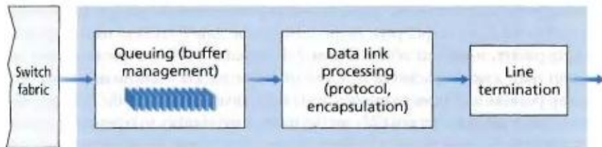
Figure 4.9 ♦ Output port processing
