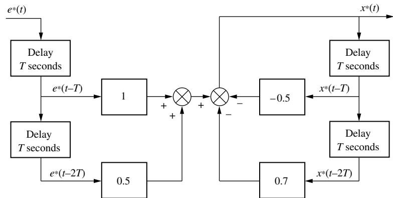
FIGURE 13.29 Flowchart to implement G_c(z) = \frac{z + 0.5}{z^2 - 0.5z + 0.7} (Reprinted with permission of John Wiley & Sons, Inc.)
