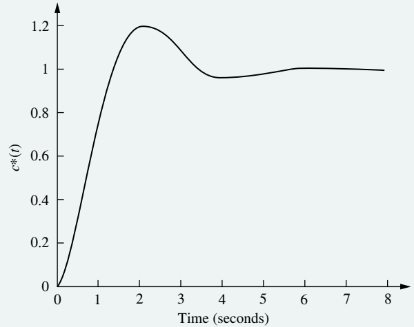
Note: Valid only at integer values of sampling instant FIGURE 13.33 Sampled step response of the antenna azimuth position control system
