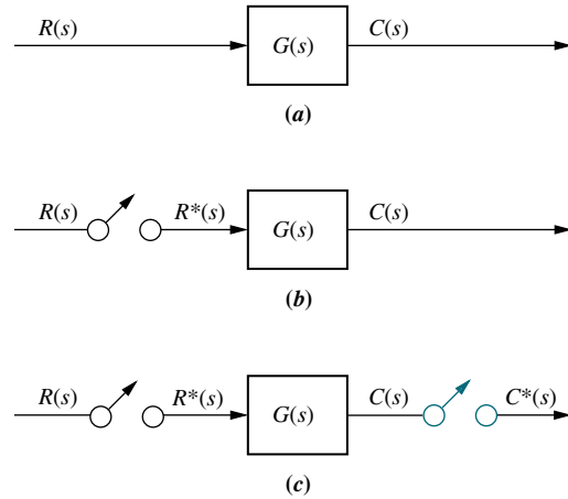
FIGURE 13.8 Sampled-data systems: a. continuous; b. sampled input; c. sampled input and output
