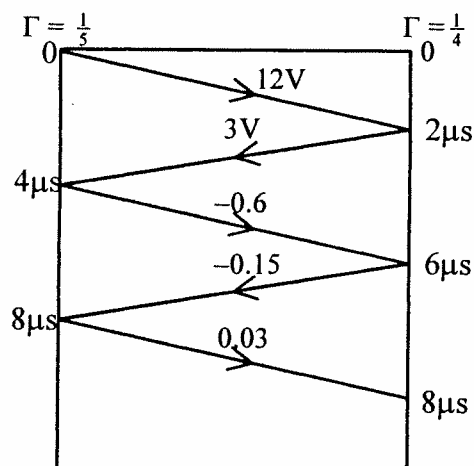
(Voltage bounce diagram)
