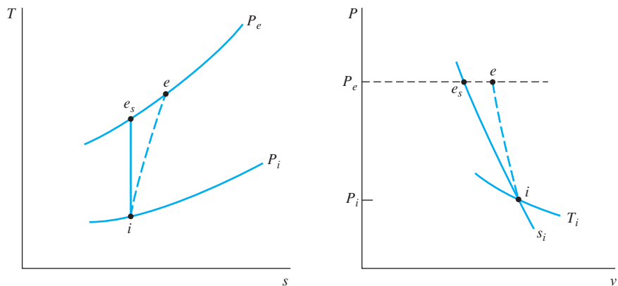
FIGURE 7.11 The compression process in an ideal and an actual adiabatic compressor.
