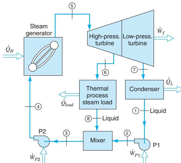
FIGURE 9.19 Example of a cogeneration system.
