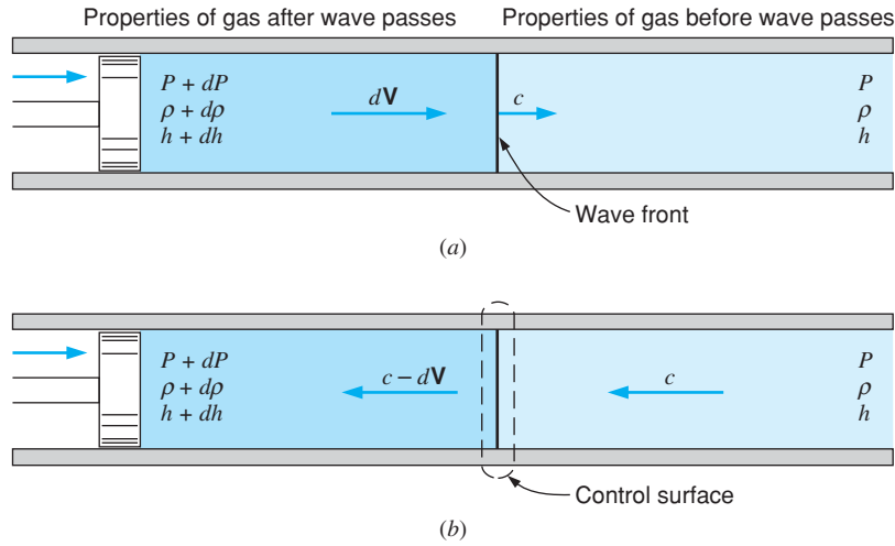
FIGURE 15.7 Diagram illustrating sonic velocity. (a) Stationary observer. (b) Observer traveling with wave front.
