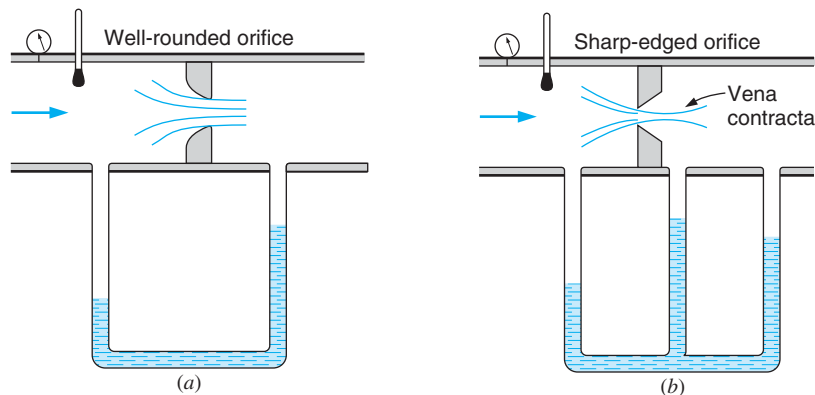
FIGURE 15.21 Nozzles and orifices as flow-measuring devices.
