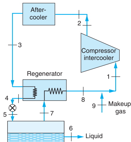
FIGURE 9.26 A Linde-Hampson system for liquefaction of gases.
