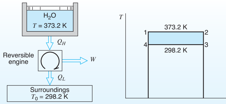
FIGURE 6.20 Reversible heat transfer with the surroundings.
