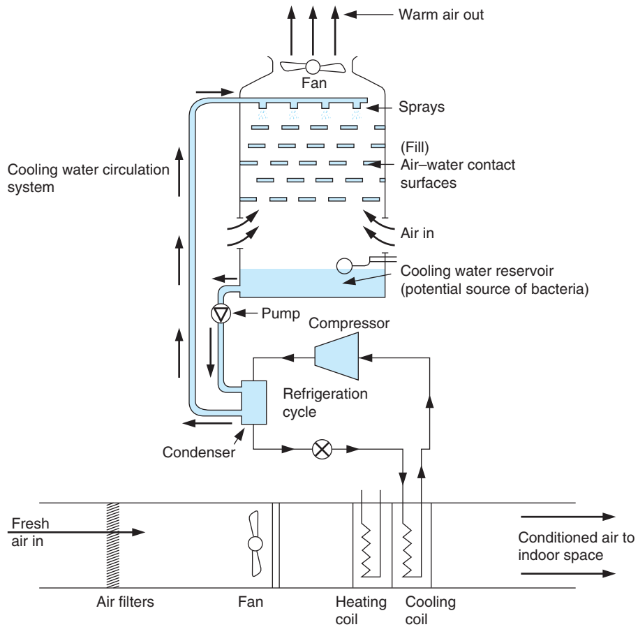
FIGURE 11.14 A cooling tower with evaporative cooling for building air-conditioning use.
