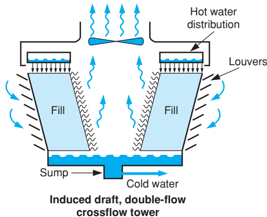
FIGURE 11.15 A cooling tower for a power plant with evaporative cooling.
