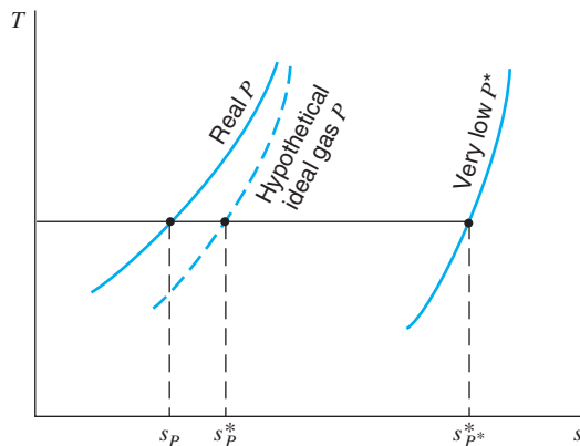
FIGURE 12.9 Real and ideal gas states and entropies.
