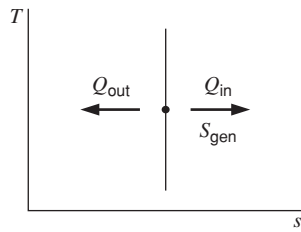
FIGURE 6.16 Change of entropy due to heat transfer and entropy generation.
