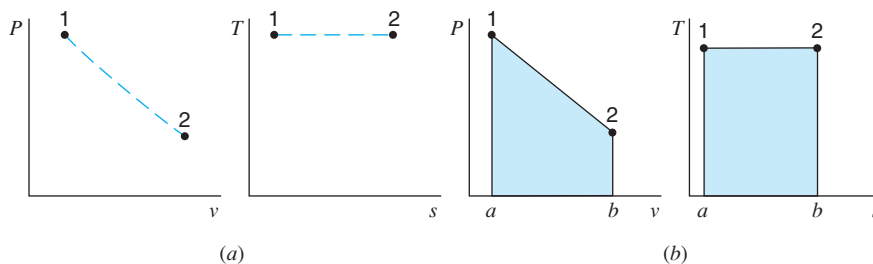
FIGURE 6.17 Reversible and irreversible processes on P-v and T-s diagrams.
