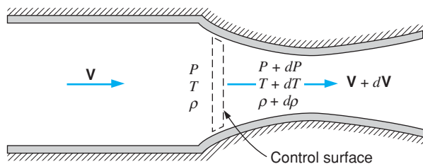
FIGURE 15.8 One-dimensional, reversible, adiabatic steady flow through a nozzle.
