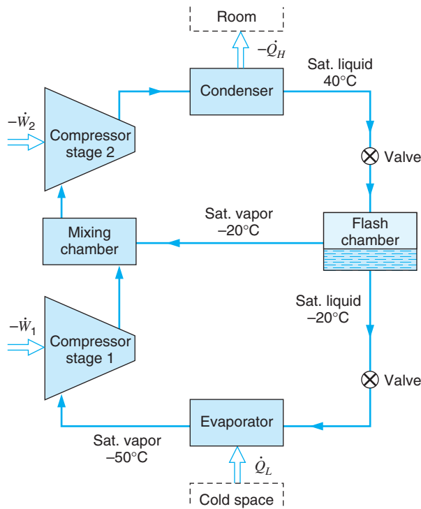
FIGURE 9.25 A two-stage compression dual-loop refrigeration system.
