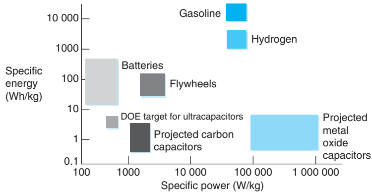
FIGURE 3.30 Specific energy versus specific power.
