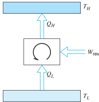
FIGURE 6.2 Reversible refrigeration cycle for demonstration of the inequality of Clausius.
