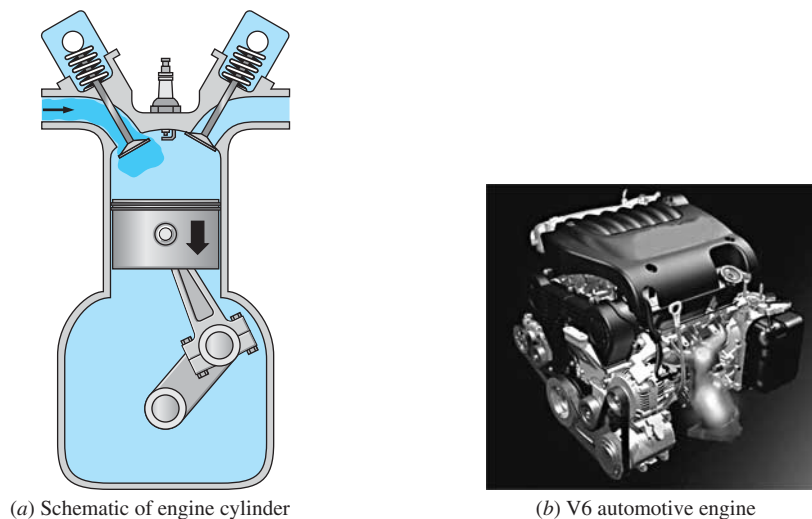
FIGURE 3.36 Schematic and photo of an automotive engine.
