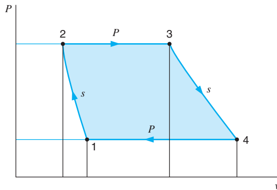
FIGURE 9.2 Four-process power cycle.
