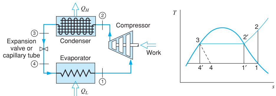
FIGURE 9.23 The ideal vapor-compression refrigeration cycle.
