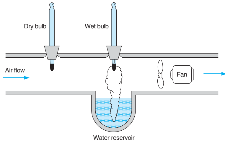
FIGURE 11.7 Steady-flow apparatus for measuring wet- and dry-bulb temperatures.
