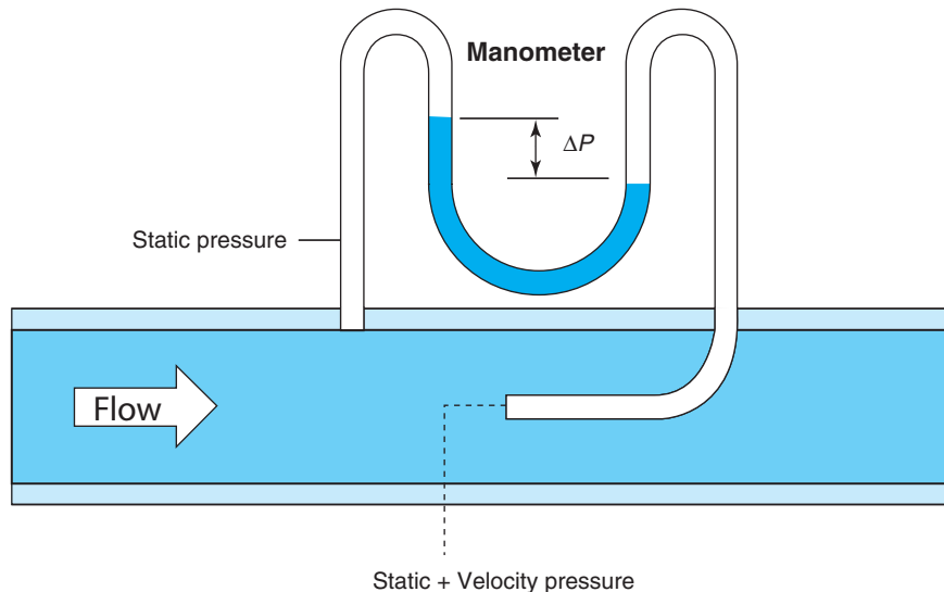
FIGURE 1.24 Schematic of flow velocity measurement.
