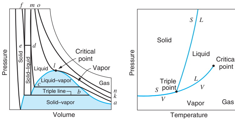
FIGURE 2.8 P - v - T surface for a substance that contracts on freezing.
