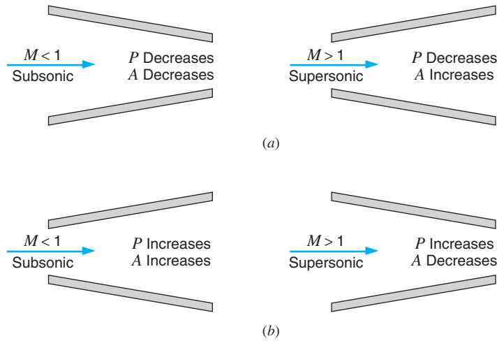
FIGURE 15.9 Required area changes for (a) nozzles and (b) diffusers.
