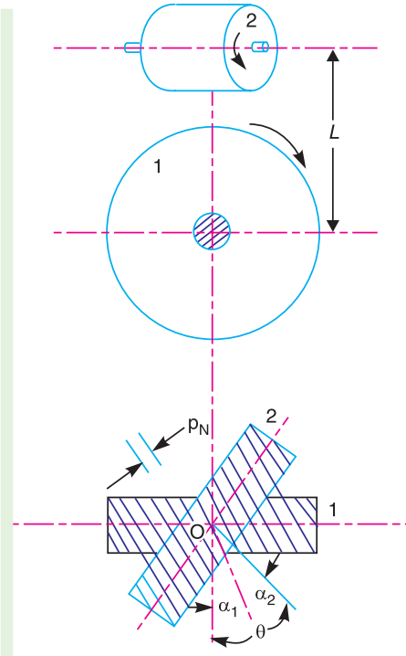
Fig. 12.16. Centre distance for a pair of spiral gears.
