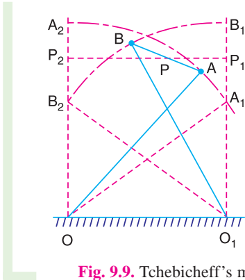
Fig. 9.9. Techebicheff's mechanism.
