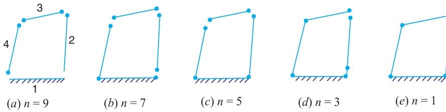
Fig. 5.15. Four bar mechanism.
