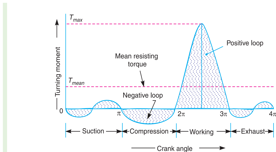
Fig. 16.2. Turning moment diagram for a four stroke cycle internal combustion engine.
