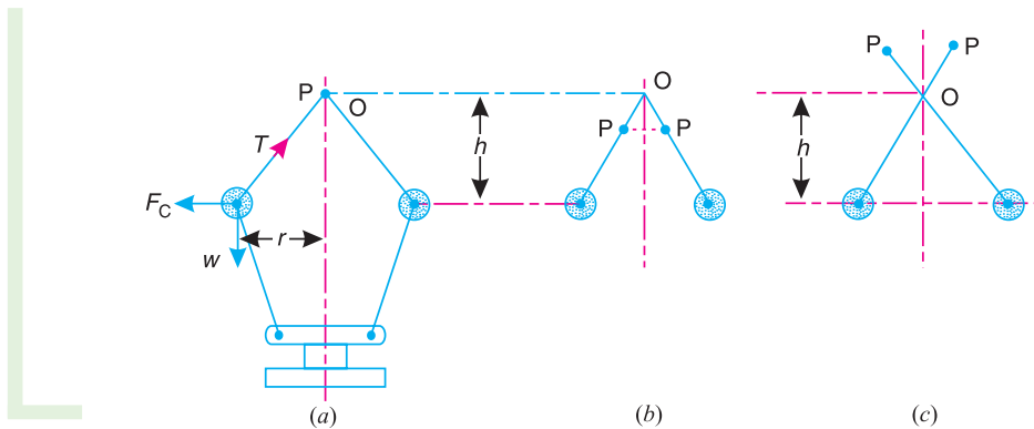
Fig. 18.2. Watt governor.
