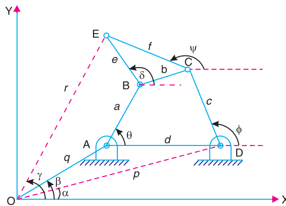
Fig. 25.16. Four bar mechanism with a couple point.
