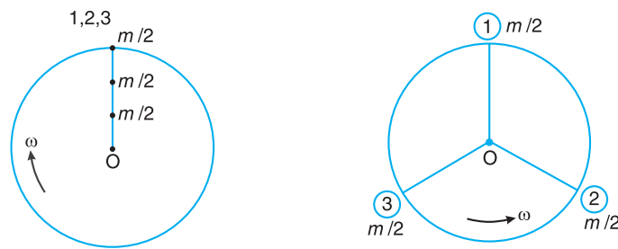
(a) Direct primary cranks. (b) Reverse primary cranks.
