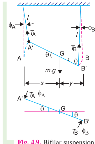
Fig. 4.9. Bifilar suspension.
