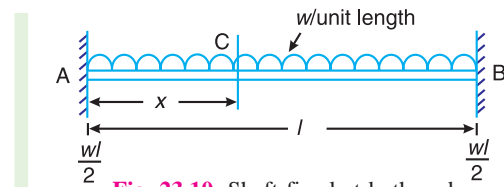
Fig. 23.10. Shaft fixed at both ends carrying a uniformly distributed load.
