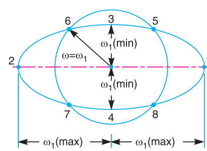
Fig. 9.20. Polar diagram-salient features of driven shaft speed.
