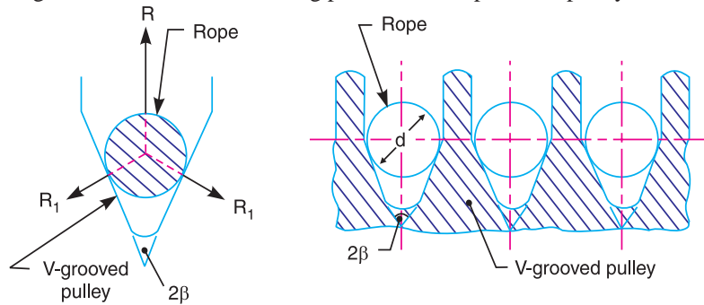
(a) Cross-section of a rope. (b) Sheave (Grooved pulley) for ropes.
