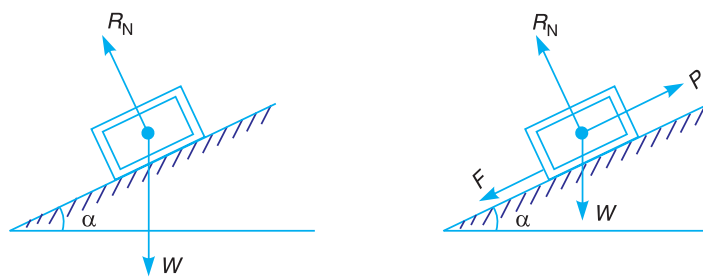
(a) Angle of inclination less than angle of friction.
