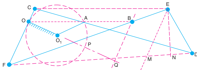
Fig. 9.4. Hart's mechanism.
