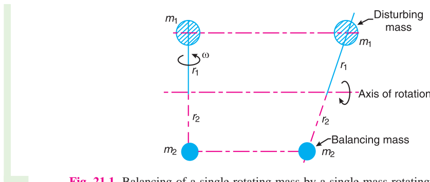
Fig. 21.1. Balancing of a single rotating mass by a single mass rotating in the same plane.
