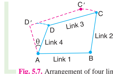
Fig. 5.7. Arrangement of four links.
