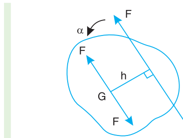
Fig. 15.1. Resultant effect of a system of forces acting on a rigid body.
