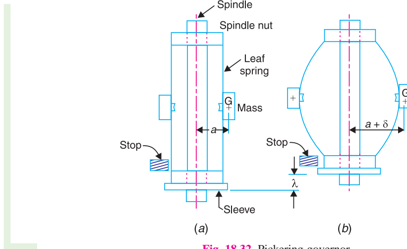
Fig. 18.32. Pickering governor.
